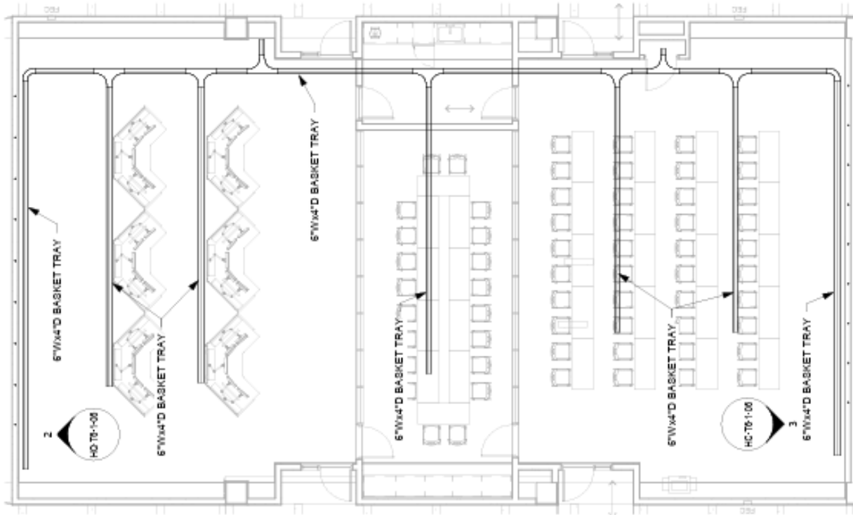
LEVEL 03 - OPERATIONS CENTER A-B - UNDER RAISED FLOOR TRAY LAYOUT
