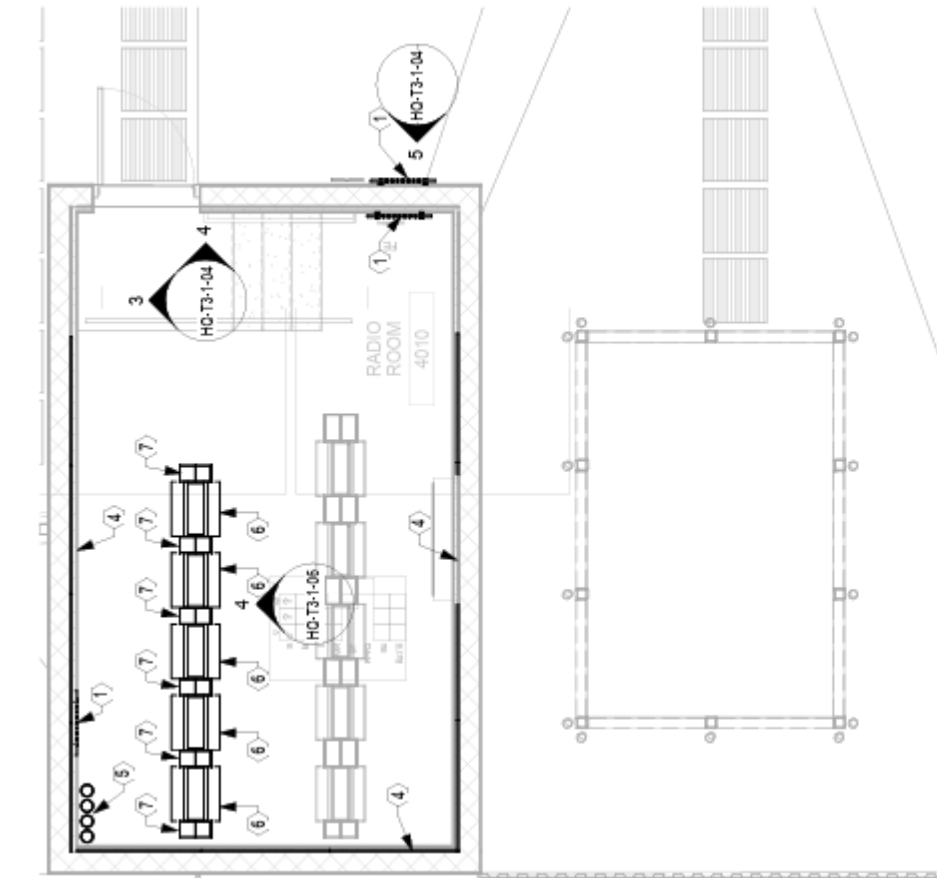
1 | HQ BLDG - RADIO RM 4010 - EQUIPMENT LAYOUT Scale: 1/4" = 1'-0"
