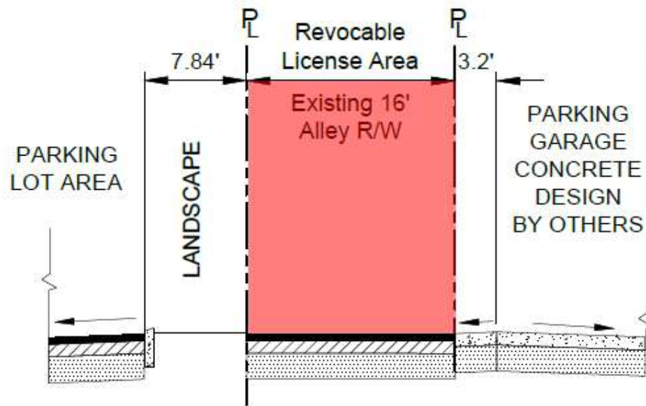
16' Alley Right-of-Way (Phases 1 & 2) - Looking East
