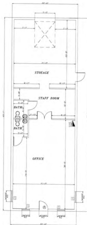
EXISTING FLOOR PLAN SCALE 1/4"=1'-0"
