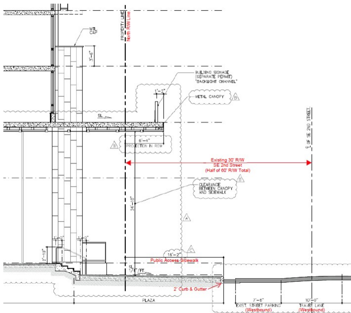
SE 2nd Street - Typical Section (Looking East)
