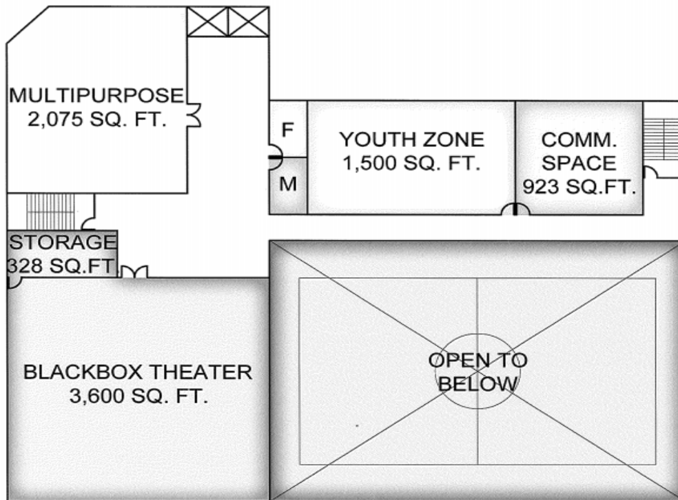
THIRD FLOOR
