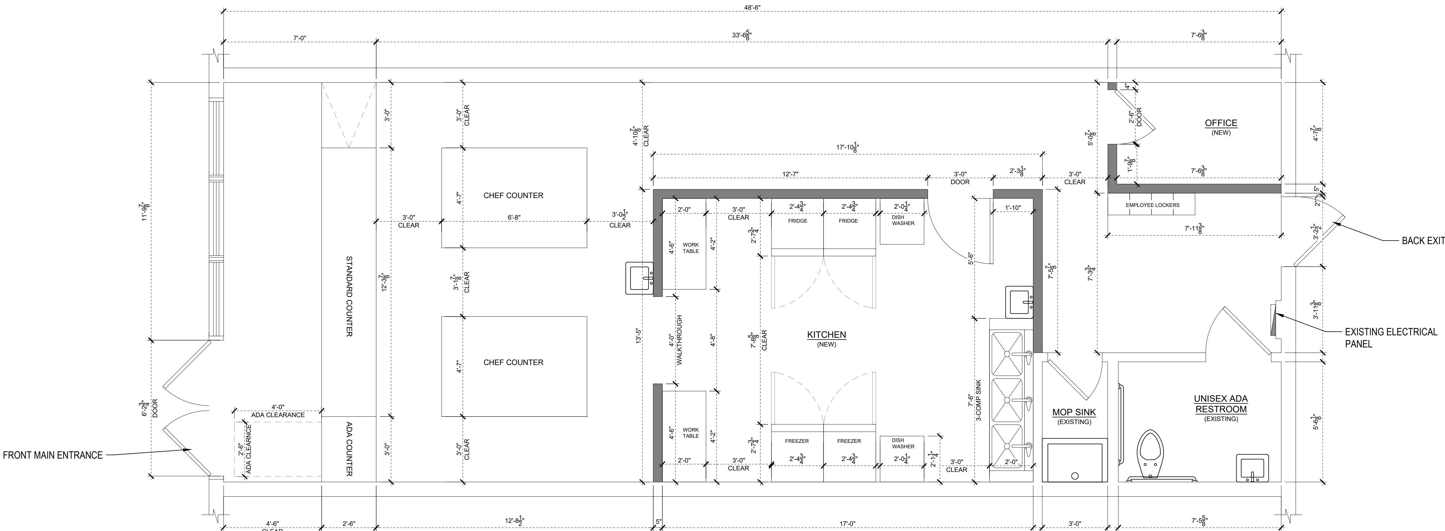
PROPOSED ELECTRICAL PLAN SCALE: 3/8"=1'-0"
