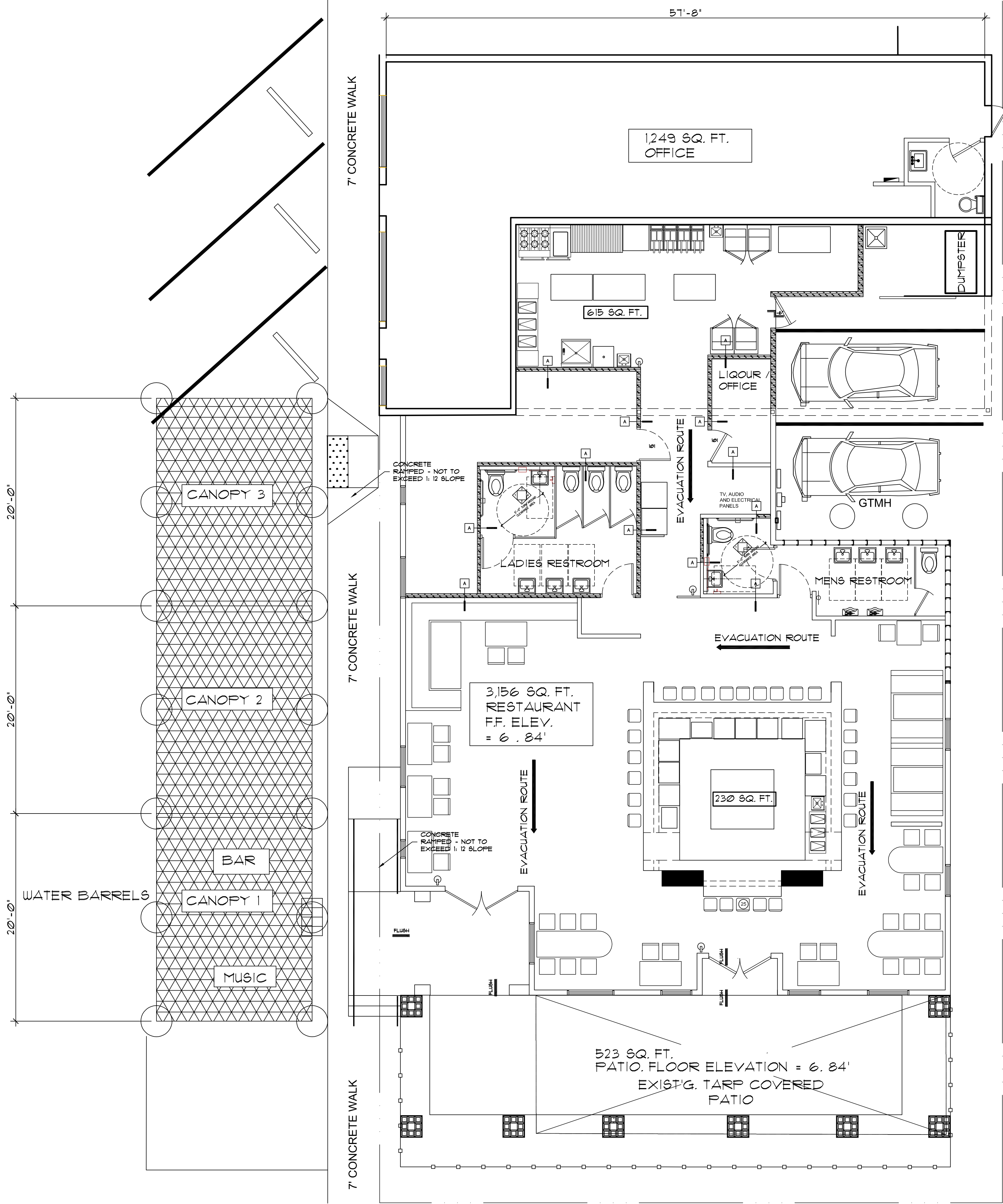
FLOOR PLAN SCALE: 3/16" = 1'-0" EXISTING 1 STORY BLDG. S-1
