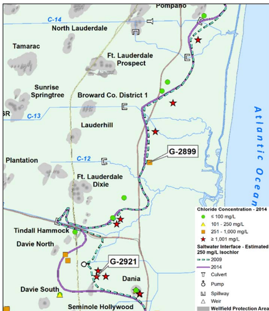
Figure 2-3: 250 mg/L Isochlor
