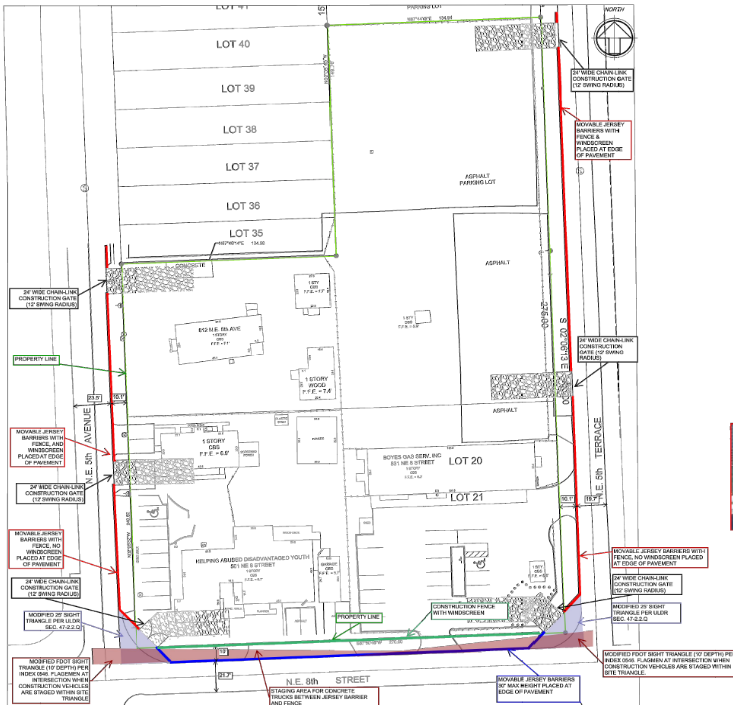
JERSEY BARRIER WITH FENCE & WINDSCREEN
