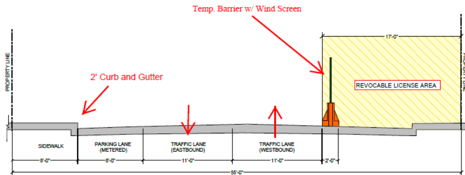
SECTION "B" - VIRAMAR STREET
