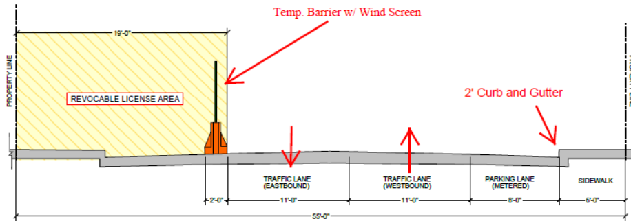
SECTION "A" - WINDMAR STREET
