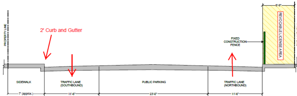
SECTION "D" - BREAKERS AVE
