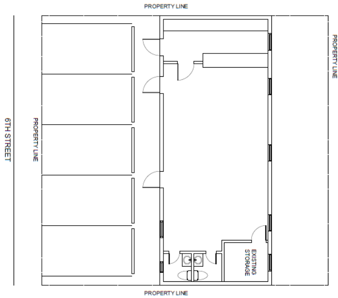
1 EXISTING FLOOR PLAN
