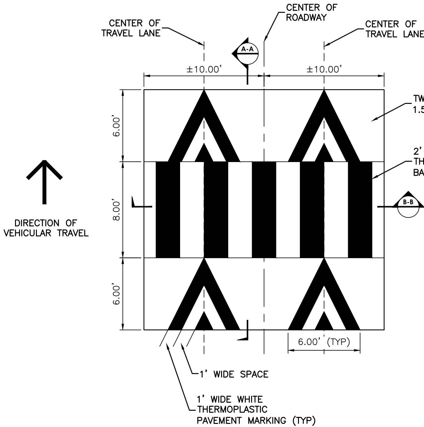
PLAN VIEW
