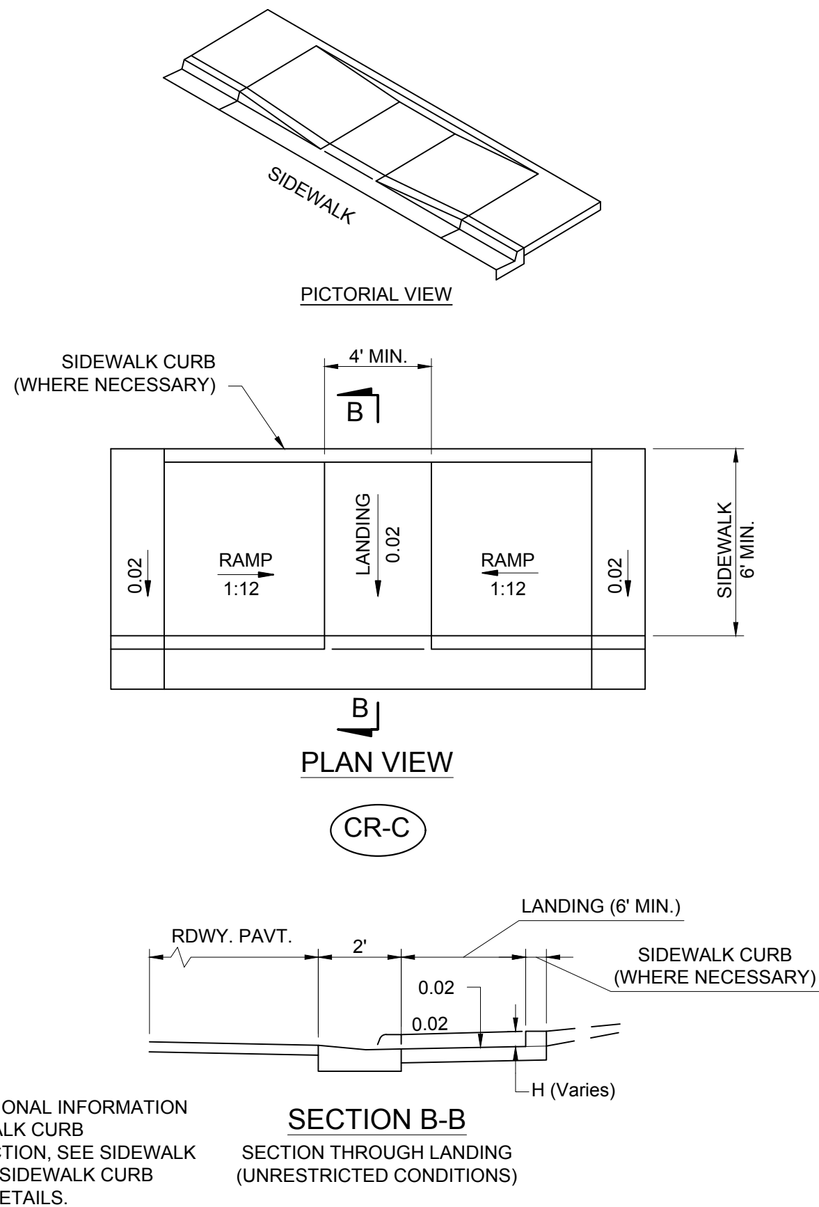
RAMP AND LANDING STRIPS NOT RESTRICTED
