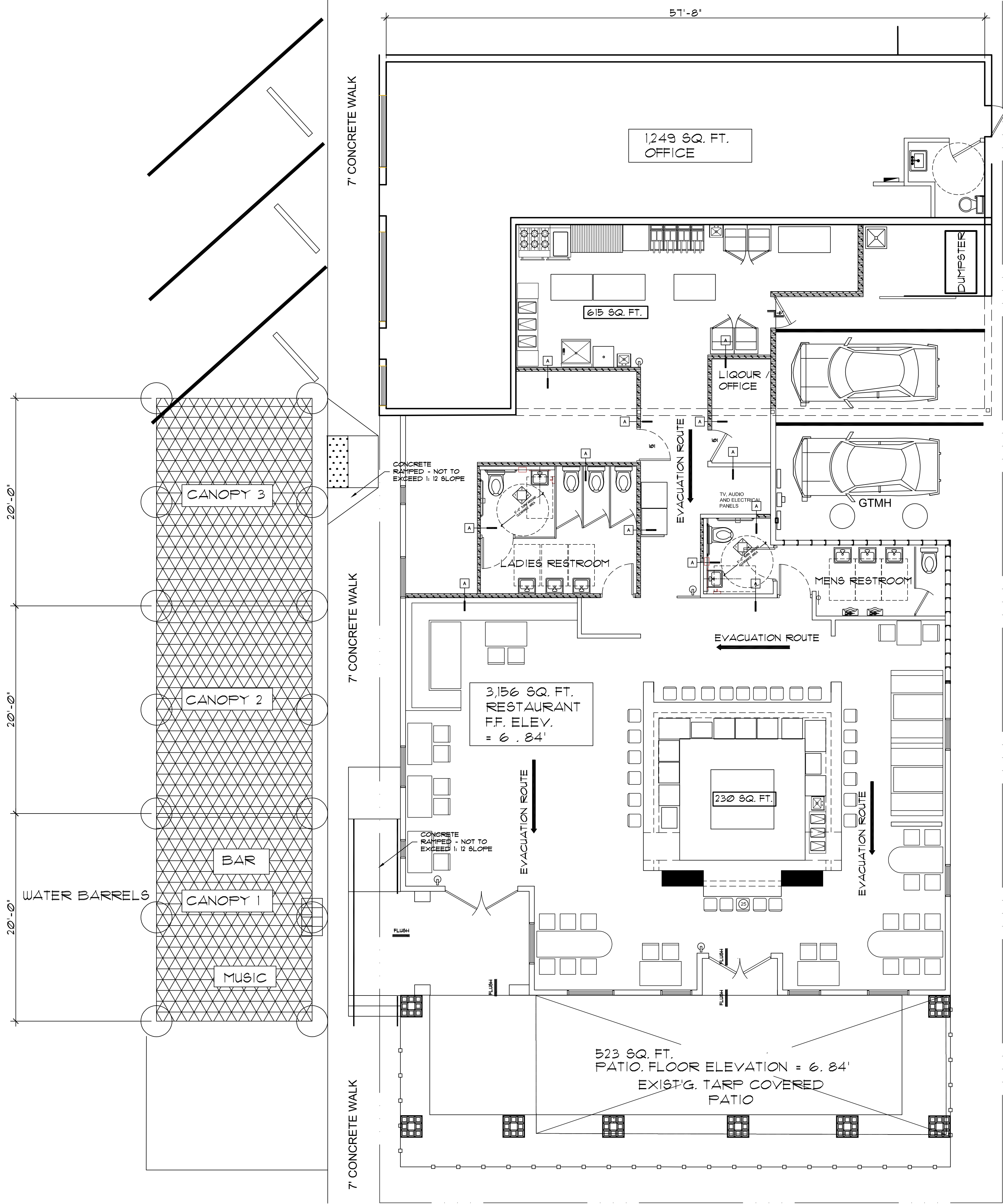
FLOOR PLAN SCALE: 3/16" = 1'-0" EXISTING 1 STORY BLDG.
