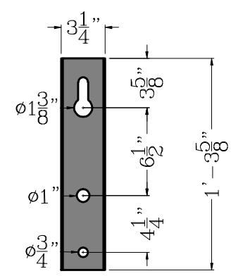
MOUNTING PLATE
