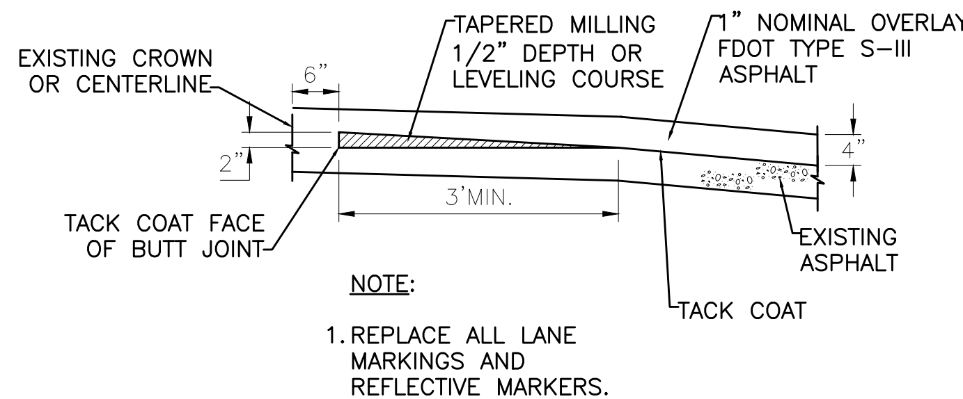
ASPHALT TAPER DETAIL
