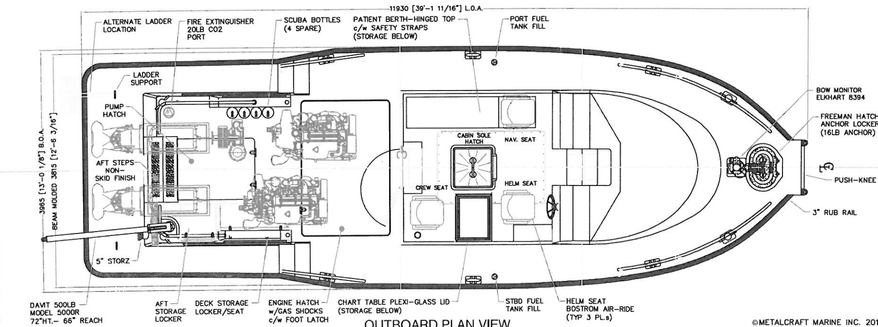
OUTBOARD PLAN VIEW
