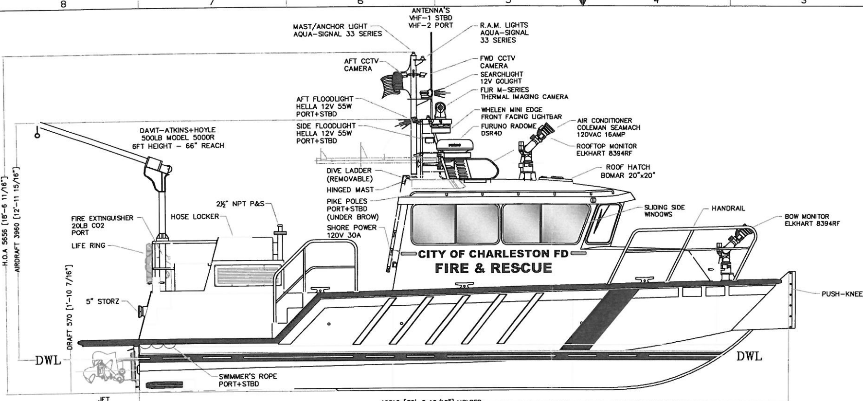
OUTBOARD PROFILE VIEW
