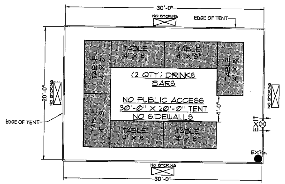
30'-0" X 20'-0" TENT FLOOR PLAN SCALE: 1/4" = 1'-0"
