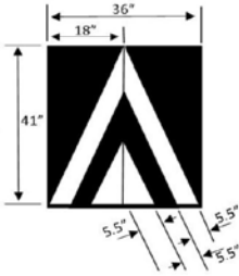
MUTCD Modified Chevron Pattern
