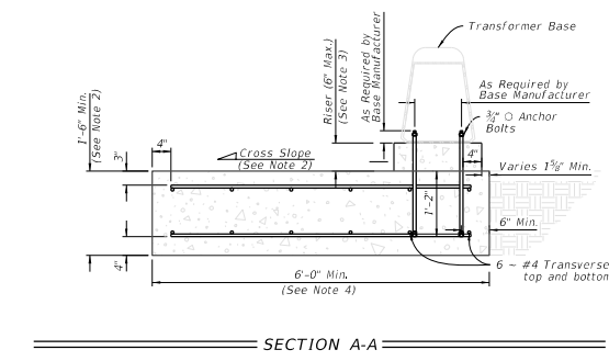
SPREAD FOOTING FOUNDATION
