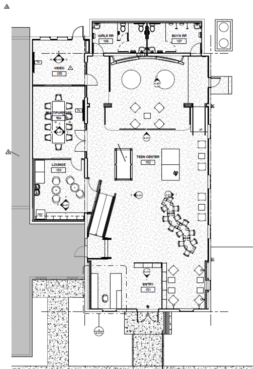
1 FIRST FLOOR PLAN - FTE 1/16" = 1'-0"
