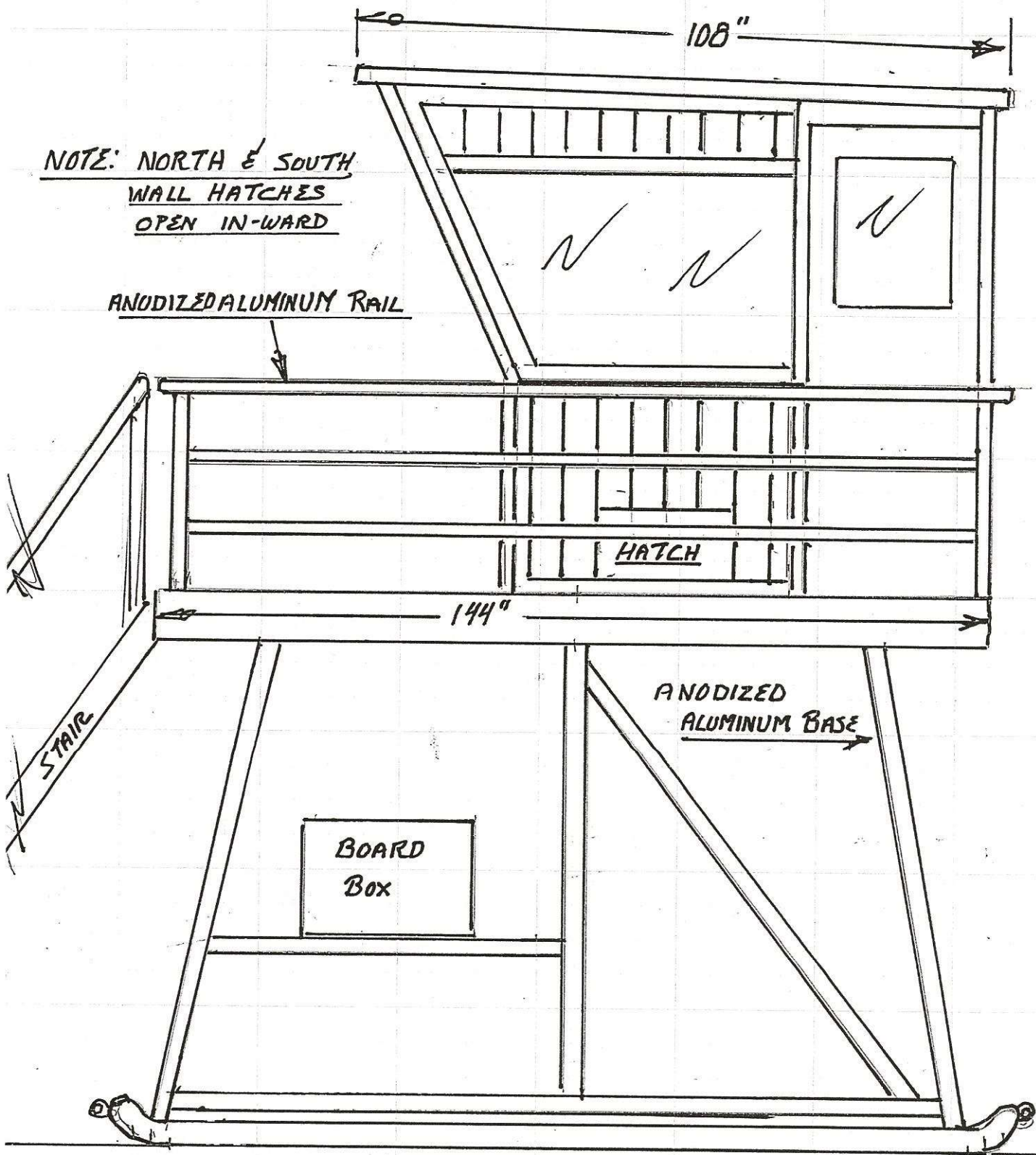
NORTH VIEW
