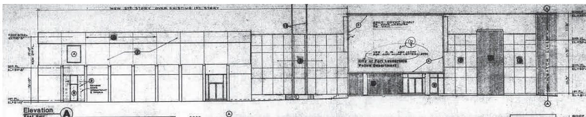
North Elevation of Police Station (1981)
