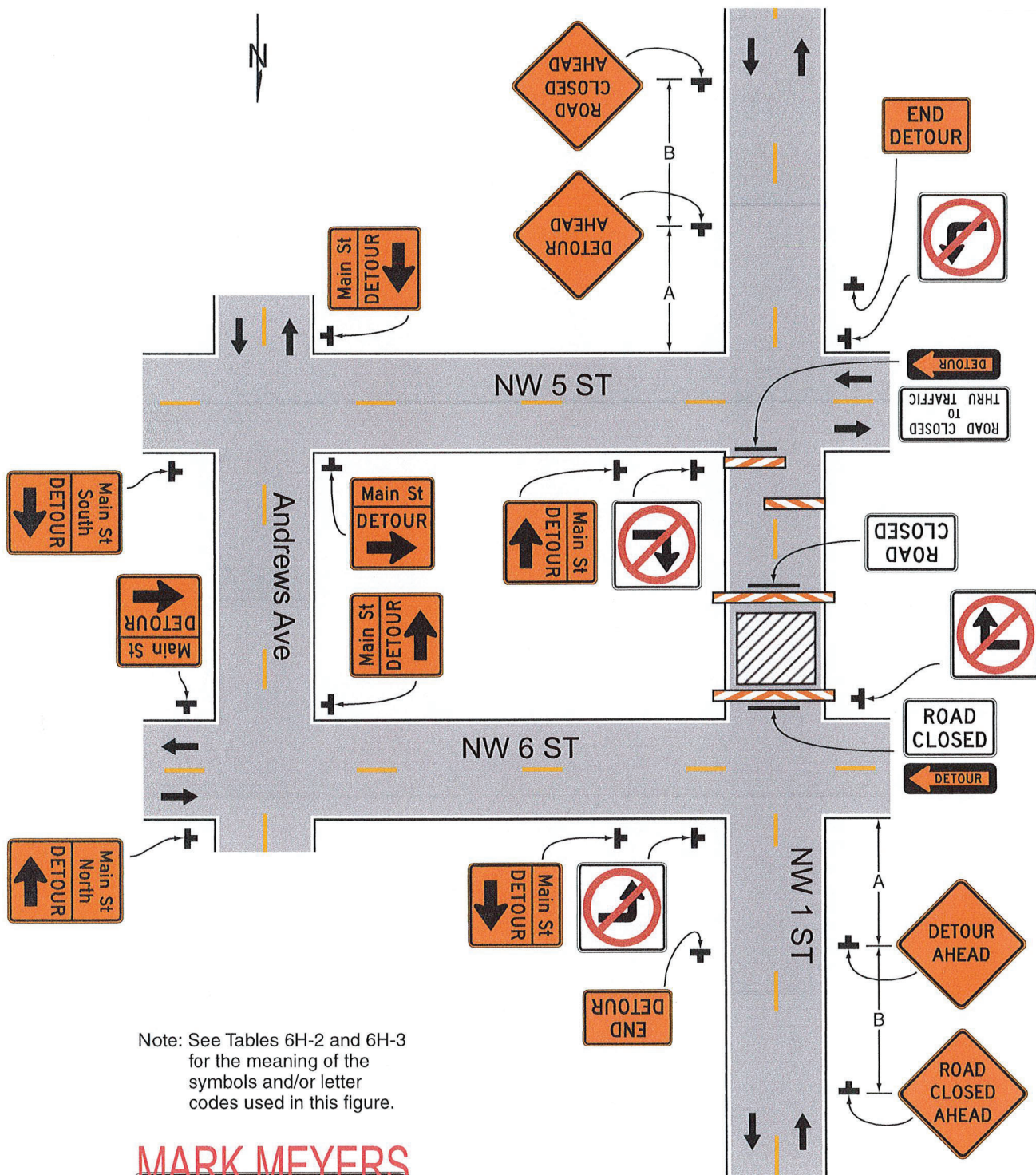
Typical Application 20
