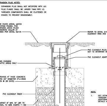
213B CLEAN-OUT COVER ASSEMBLY FOR 4-INCH OR 6-INCH CLEANOUTS N.T.S.
