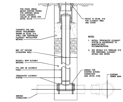
215 TRENCHLESS CLEANOUT SYSTEM FOR INSTALLATION ON 4-INCH AND 6-INCH SANITARY SERVICE CONNECTIONS N.T.S.
