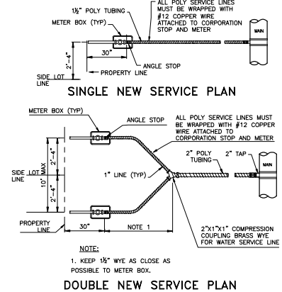
TYPICAL WATER SERVICE (301)
