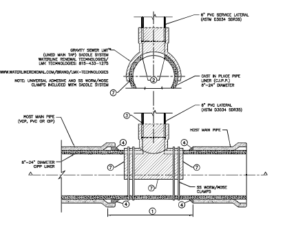
217 SADDLE TEE FASTENED TO LINED GRAVITY MAIN N.T.S.
