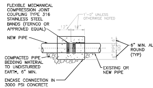
211 JOINT FOR DISSIMILAR GRAVITY SEWER PIPE N.T.S.
