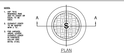
216 CLEANOUT RING AND COVER N.T.S.
