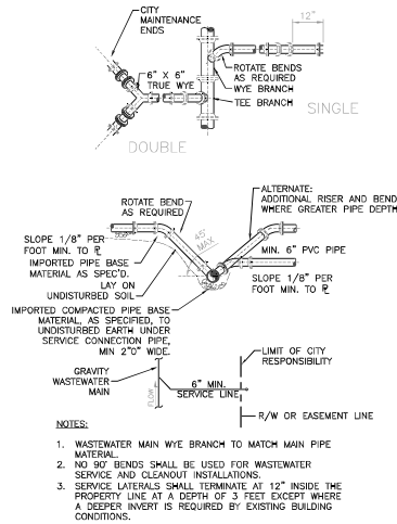
208 TYPICAL WASTEWATER SERVICE CONNECTION N.T.S.
