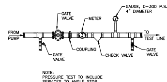
PRESSURE TEST DETAIL (306)
