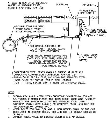
TYPICAL WATER SERVICE INSTALLATION (300)
