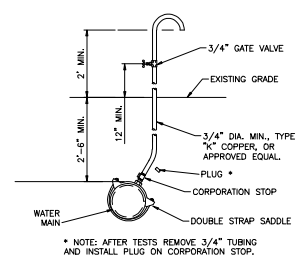
TYPICAL BACTERIOLOGICAL SAMPLING POINT AT INTERMEDIATE POINTS (304)
