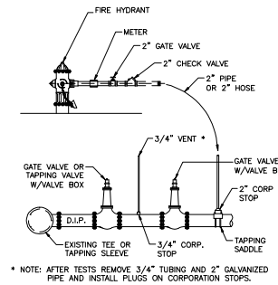
FILLING CONNECTION (305)
