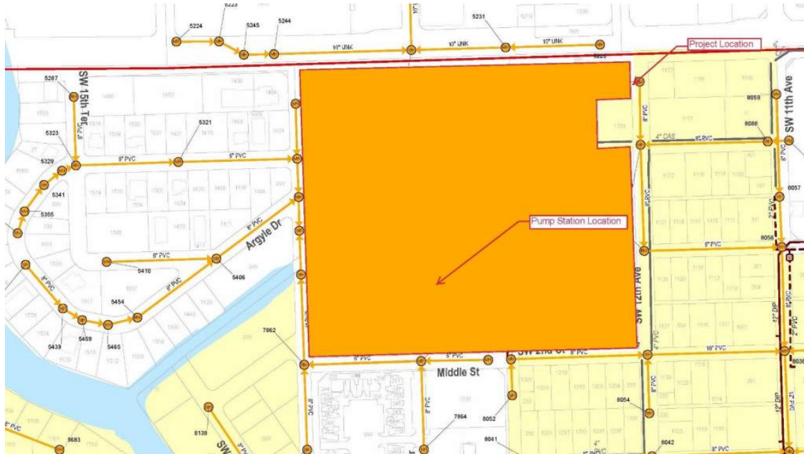
Figure 2 – City Sewer Atlas
