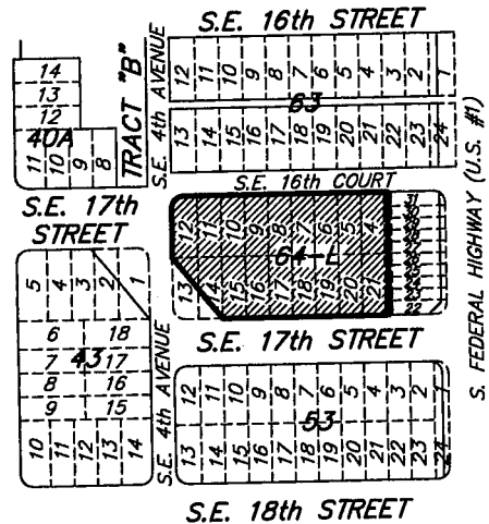
S.E. 18th STREET BLOCK PLAN NOT TO SCALE
