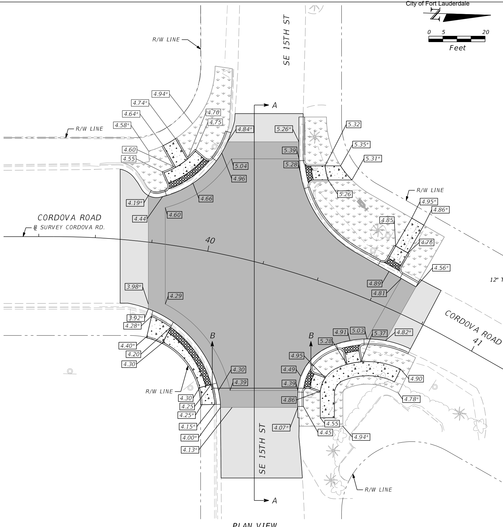
PLAN VIEW
