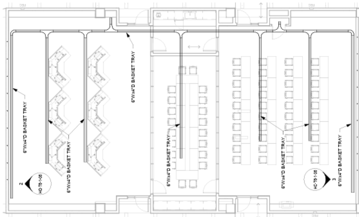
LEVEL 03 - OPERATIONS CENTER A-B - UNDER RAISED FLOOR TRAY LAYOUT Scale: 1/8" = 1'-0"
