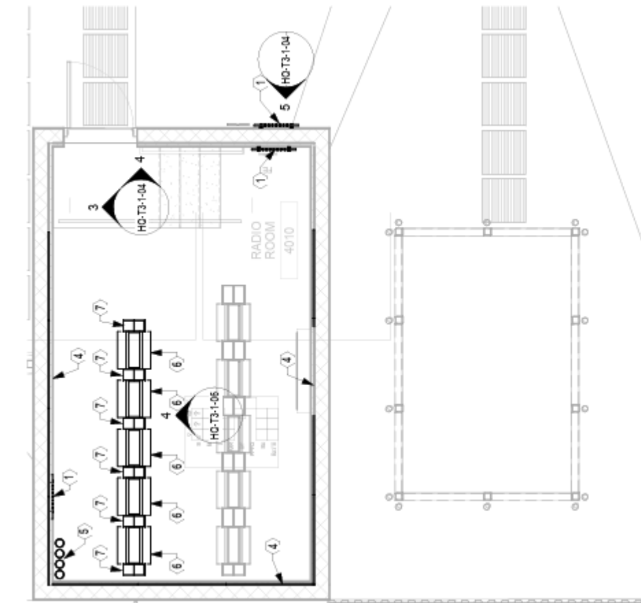
1 | HQ BLDG - RADIO RM 4010 - EQUIPMENT LAYOUT HQ-T2-1-4D | Scale: 1/4" = 1'-0"
