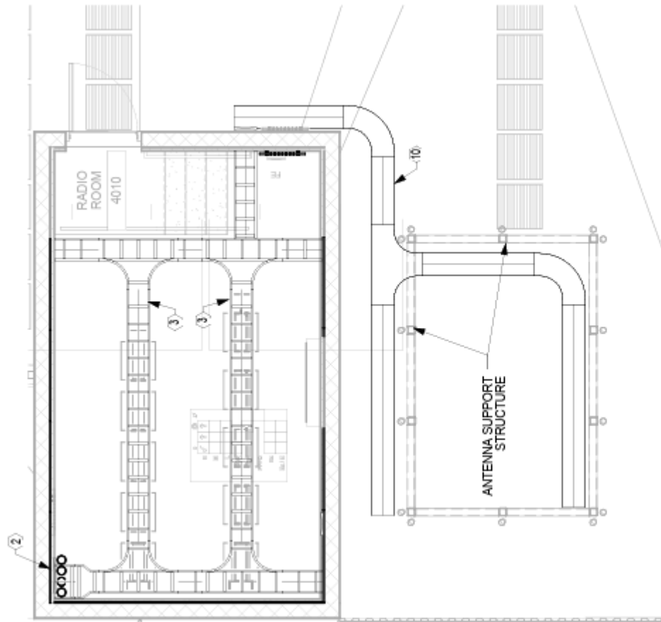
2 | HQ BLDG - RADIO RM 4010 - CABLE PATHWAY LAYOUT Scale: 1/4" = 1'-0"
