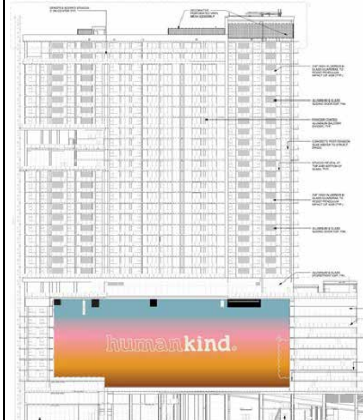
EAST ELEVATION - PROPOSED (2025)
