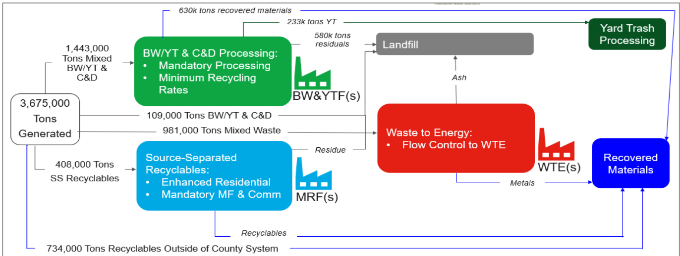
Figure 27: Schematic of Projected Scenario C Material Flow in 2025
