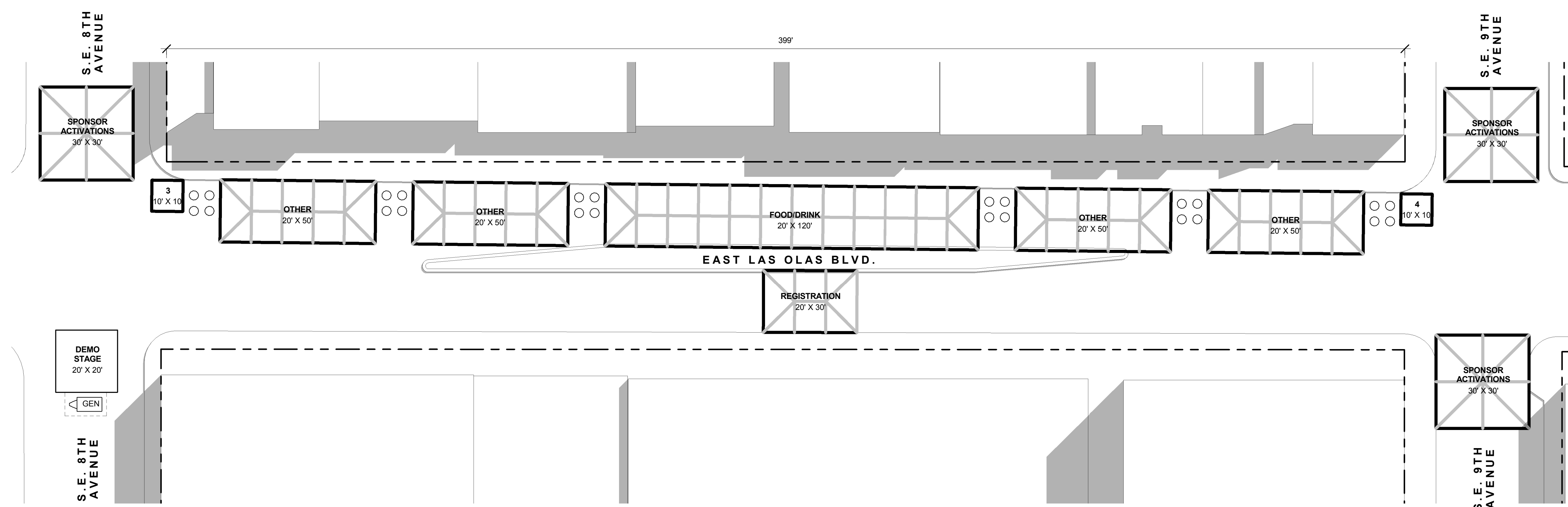
① 800 BLOCK PLAN 1" = 20'-0"
