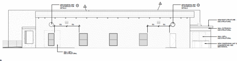
1 SOUTH ELEVATION 3/16" = 1'-0"
