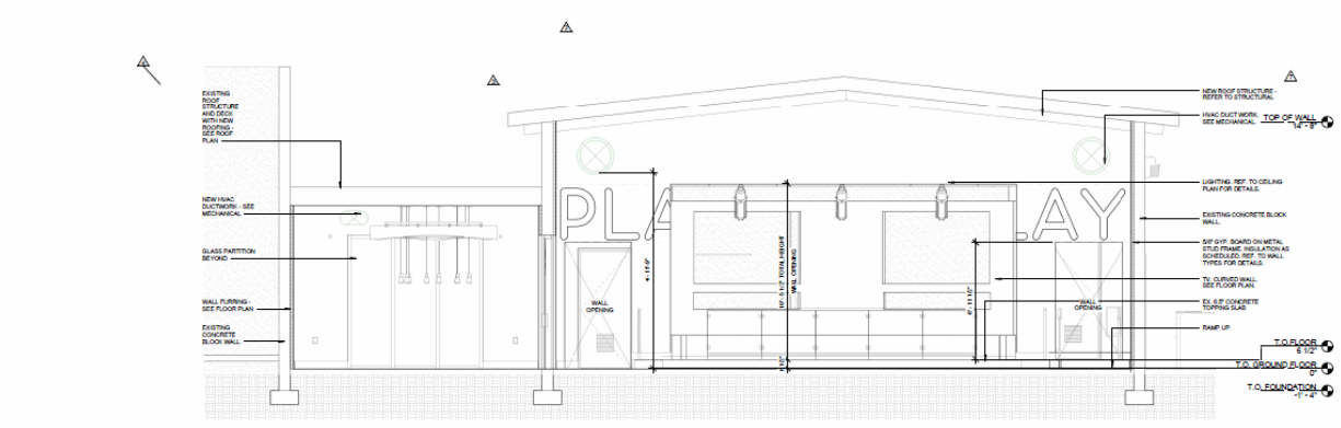
1 BUILDING SECTION - TEEN CENTER AND LOUNGE
