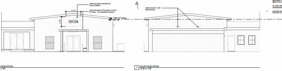
1 NORTH ELEVATION 3/16" = 1'-0"
