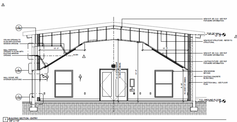
2 BUILDING SECTION - ENTRY
