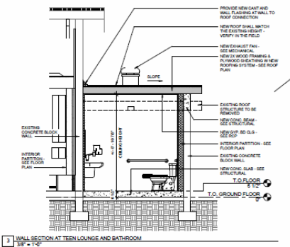
3 WALL SECTION AT TEEN LOUNGE AND BATHROOM
