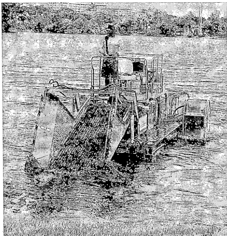
Harvester
