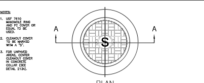
216 CLEANOUT RING AND COVER N.T.S.
