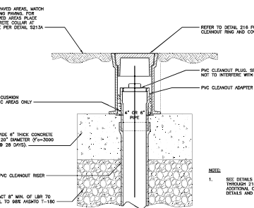
214 CLEAN-OUT COVER ASSEMBLY FOR 4-INCH OR 6-INCH CLEANOUTS N.T.S.
