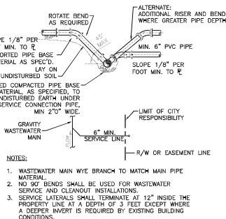
208 TYPICAL WASTEWATER SERVICE CONNECTION N.T.S.
