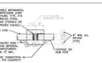
210 NEW LATERAL ON EXISTING GRAVITY WASTEWATER MAIN N.T.S.
