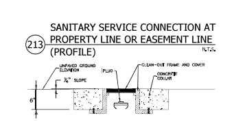
213A CONCRETE COLLAR FOR CLEANOUTS IN UNPAVED AREAS N.O.C.
