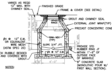
202 INVERT FLOW CHANNELS N.T.S.
