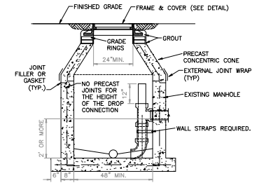
206 OUTSIDE DROP CONNECTION PRECAST MANHOLE - TYPE B N.T.S.
