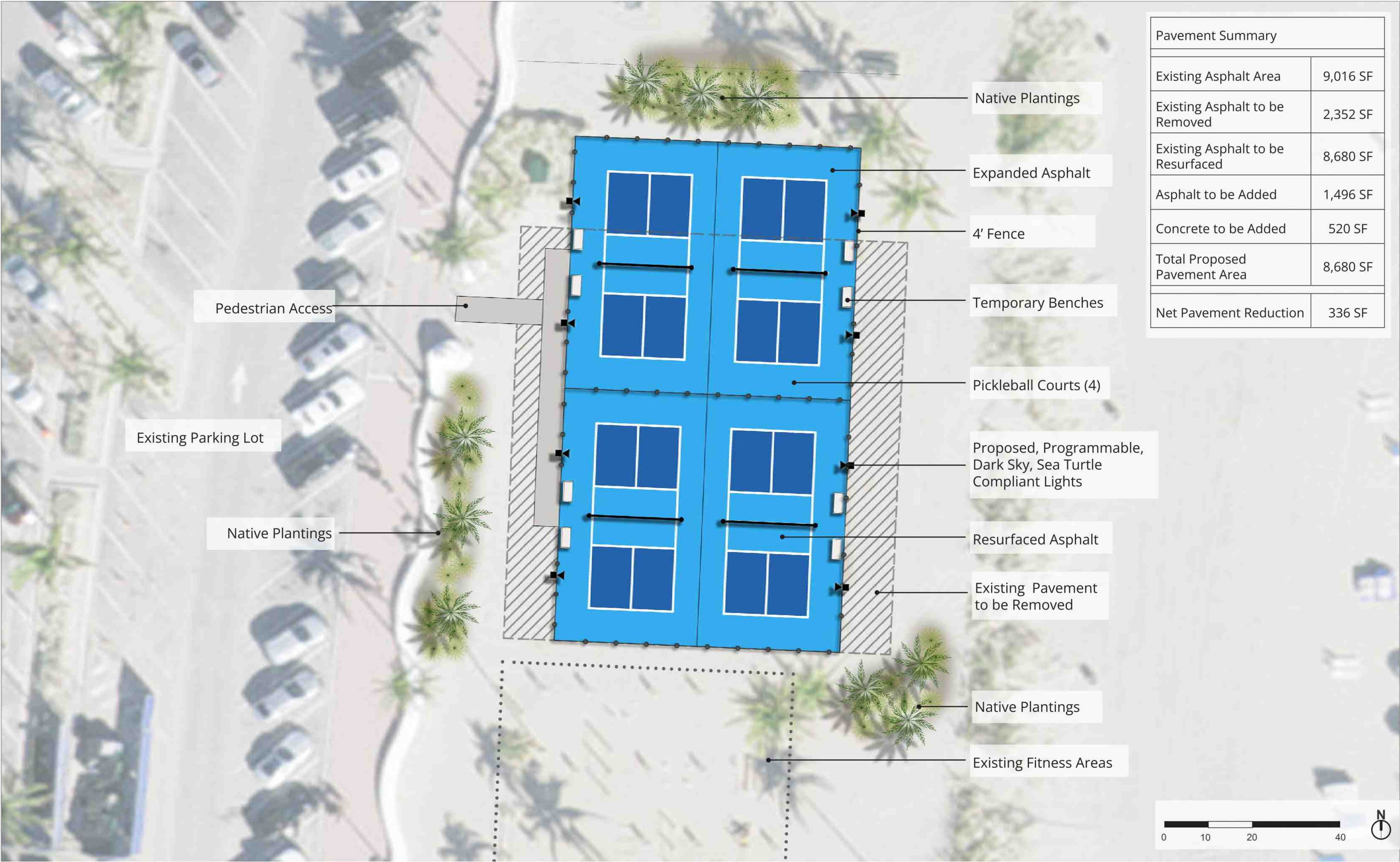
Fort Lauderdale Beach - Pickleball Courts - Initial Concept Plan - Alternative 2
