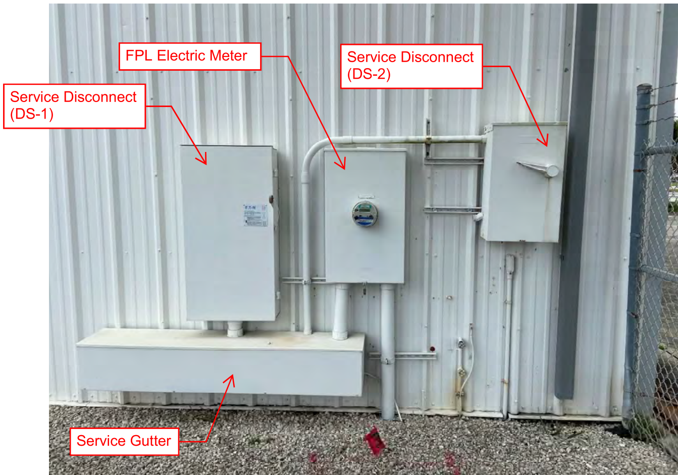
Picture 1 – Electric Meter and Service Equipment
