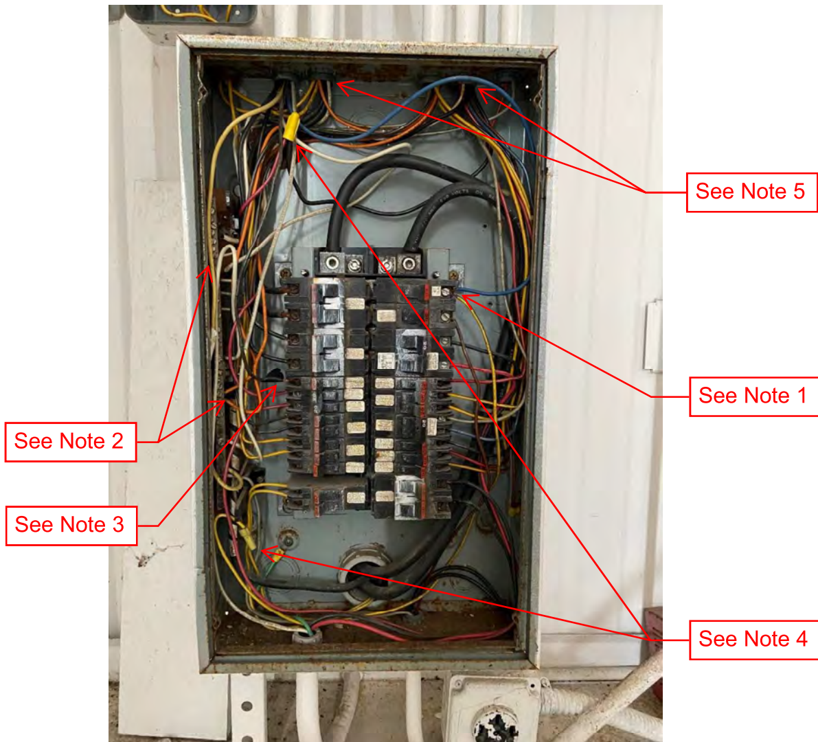
Picture 6 - Branch Circuit Conductors Panel 2
