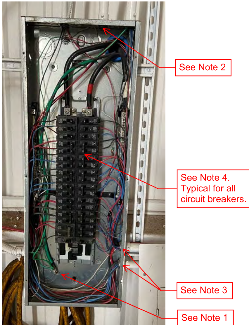
Picture 5 - Branch Circuit Conductors Panel 1
