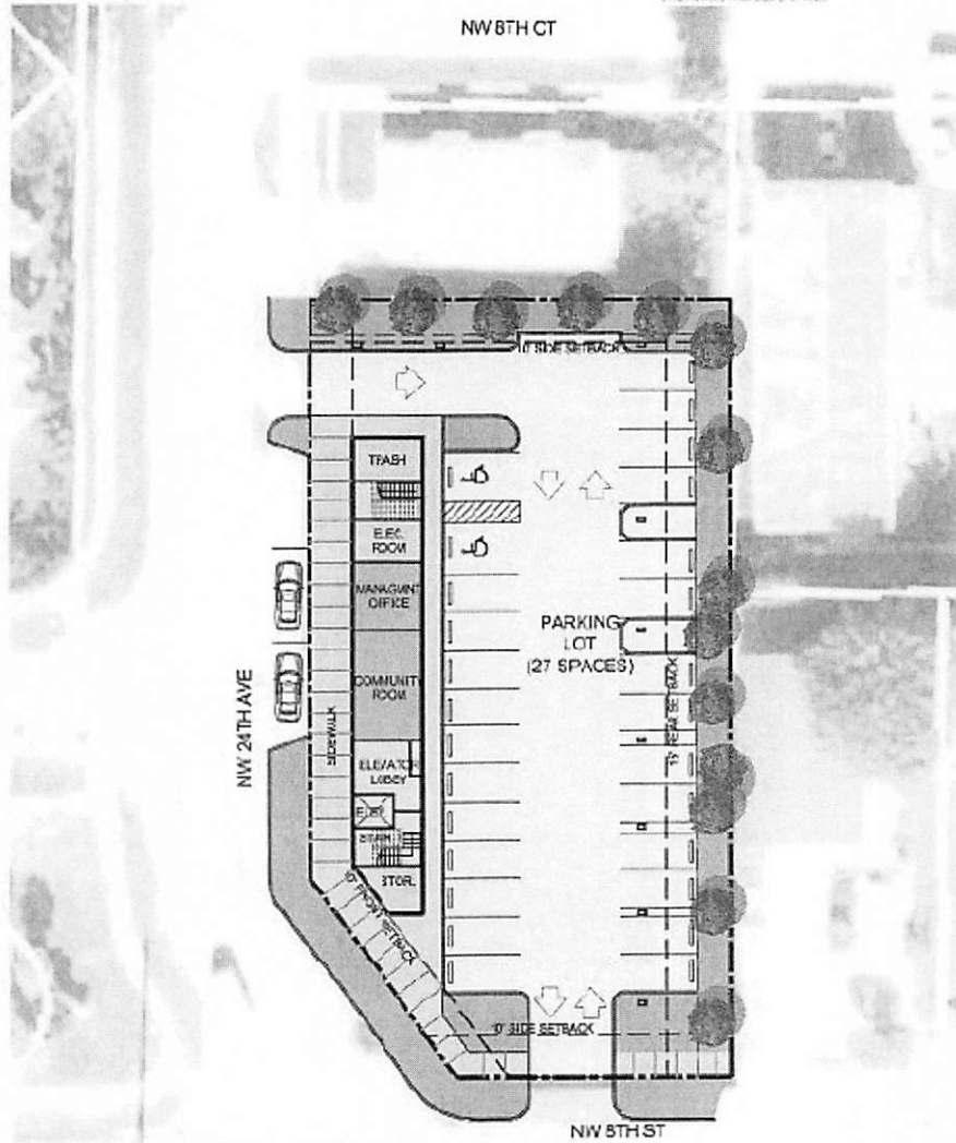
① CONCEPTUAL MASSING SITE PLAN / 1ST FLOOR PLAN SCALE: 1/8" = 1'-0"
