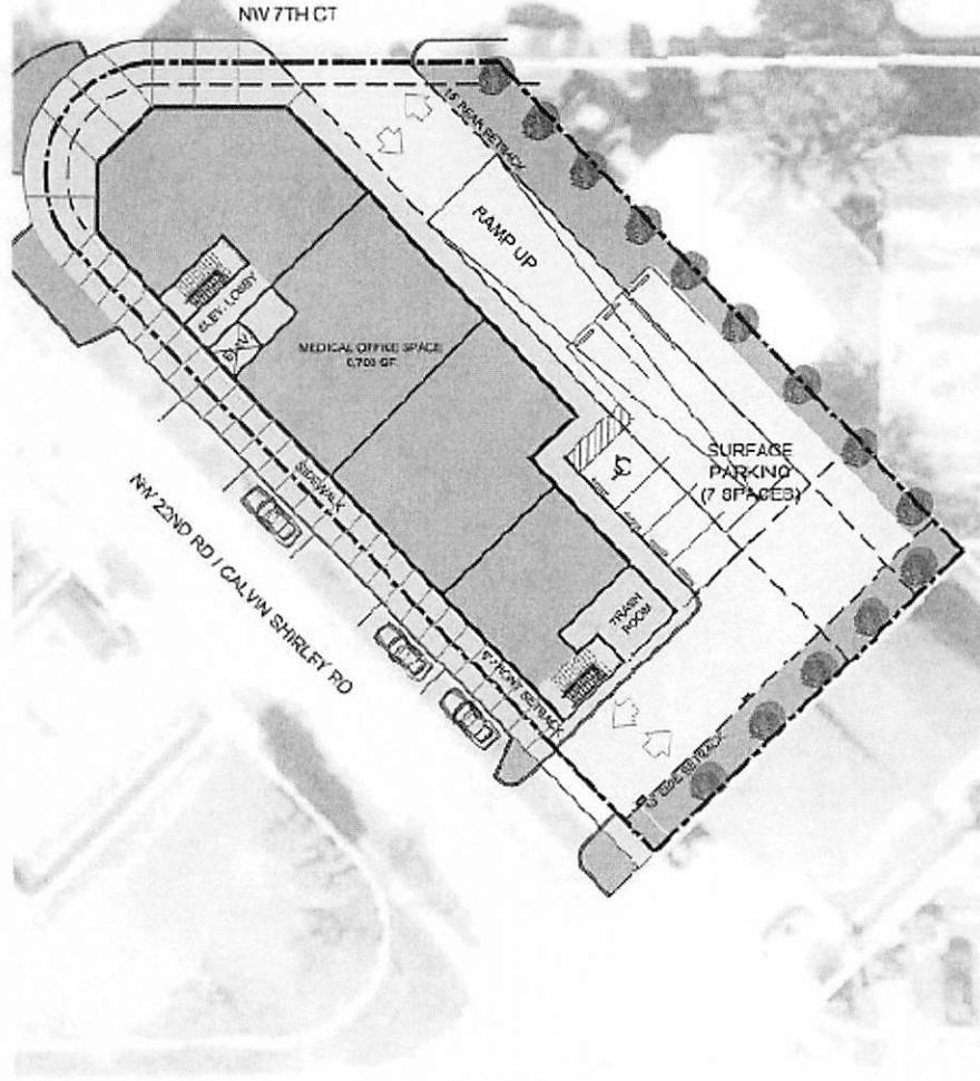
CONCEPTUAL MASSING SITE PLAN / 1ST FLOORPLAN SCALE: 1/32" = 1'-0"
