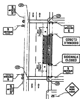
SIDEWALK DETOUR
