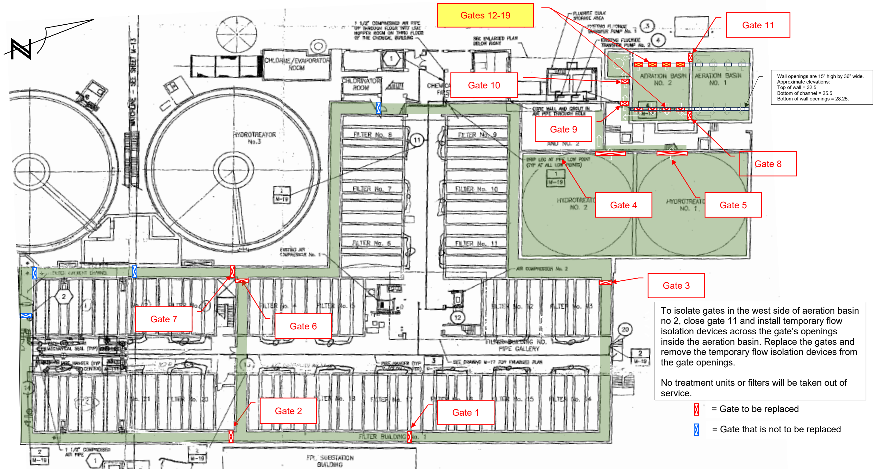
Drawing Two: Isolation Plan for Sluice Gate Replacements
