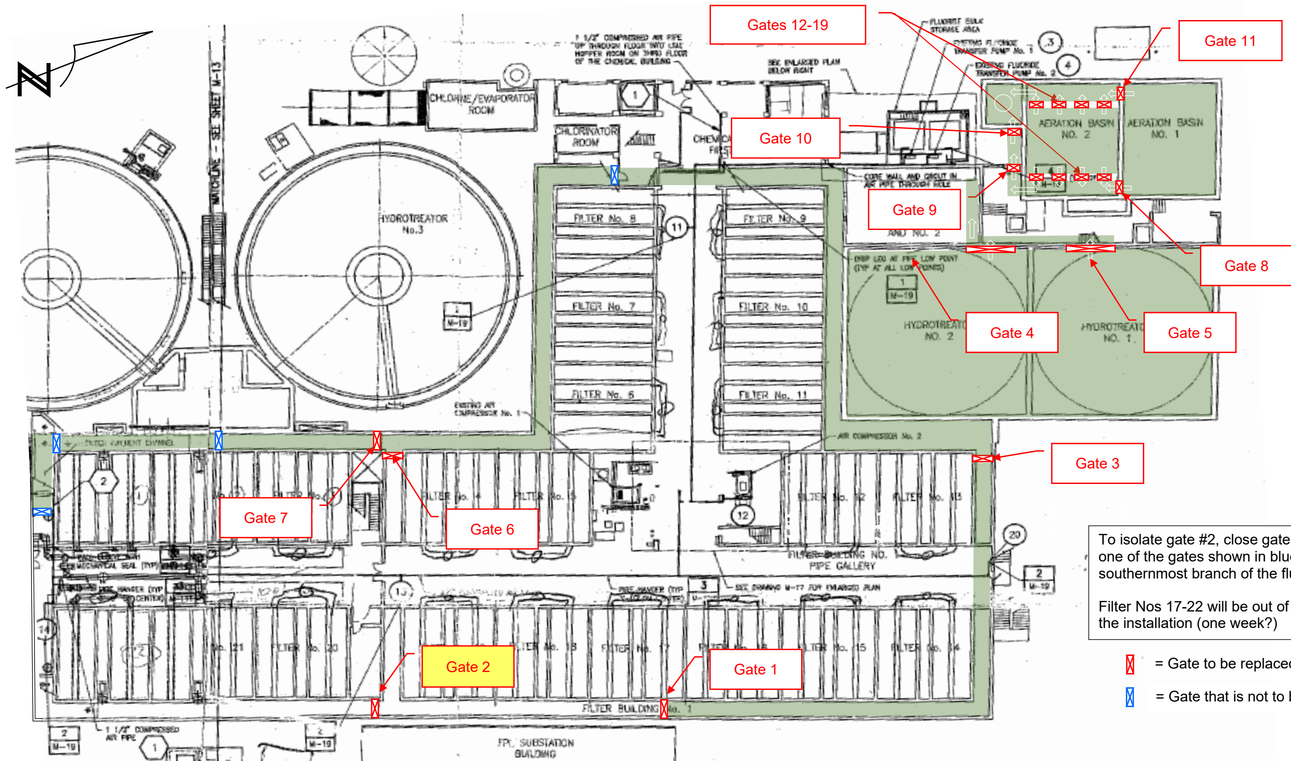
Drawing Two: Isolation Plan for Sluice Gate Replacements
