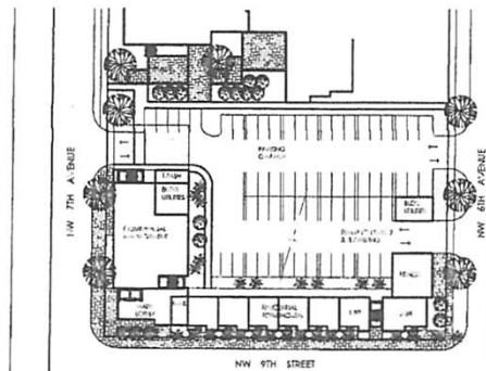
SCHEMATIC SITE & GROUND FLOOR PLAN
