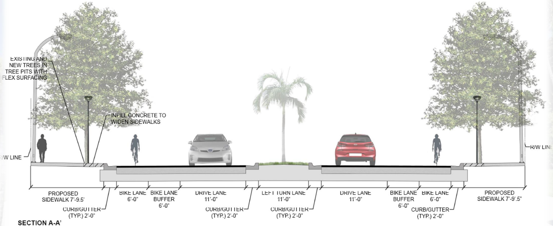
PROPOSED TYPICAL SECTION N.E. 4TH AVENUE SUNRISE BOULEVARD TO NE 13TH STREET FORT LAUDERDALE
