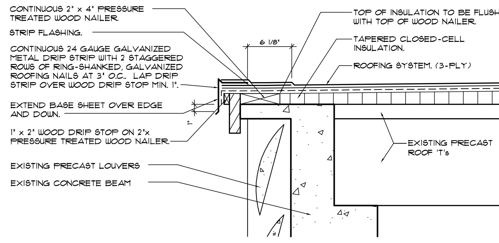
2 ROOF EDGE DETAIL AT CONCRETE DECK SCALE: 1/2" = 1'-0"
