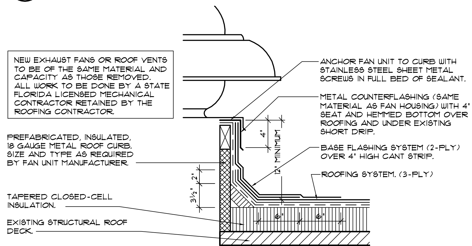
3 EXHAUST FAN OR ROOF VENT DETAIL SCALE: 1/2" = 1'-0"
