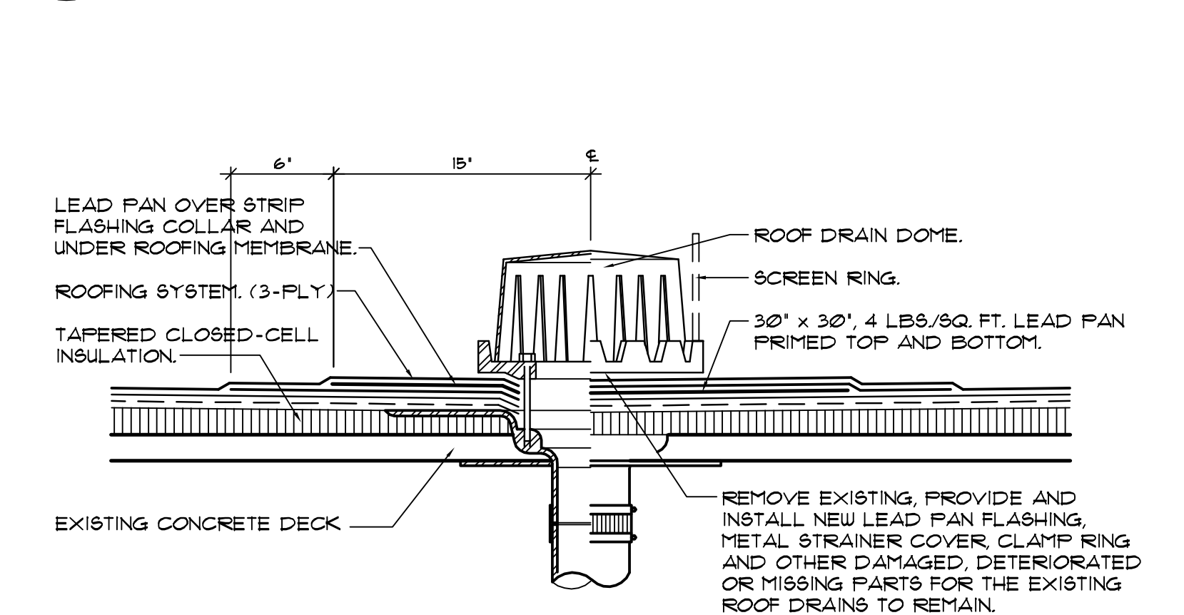
4 ROOF DRAIN DETAIL SCALE: 1/2" = 1'-0"
