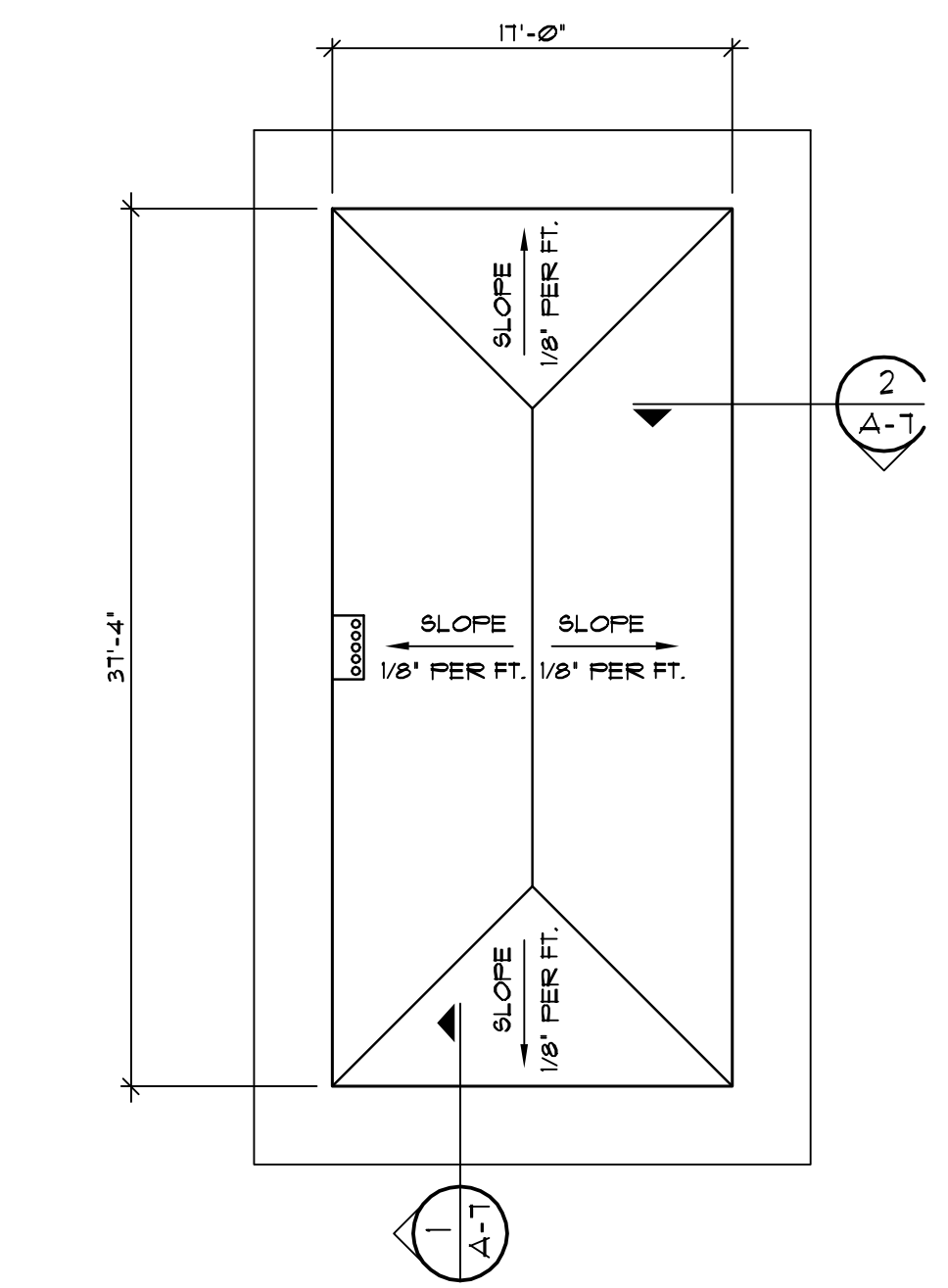
ROOF PLAN BUILDING 'F' SCALE: 1/8" = 1'-0"
