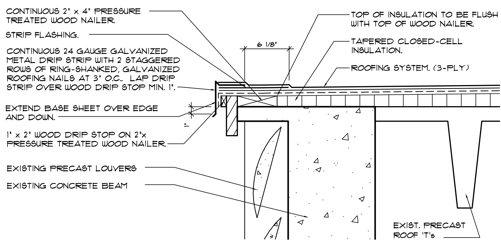
1 ROOF EDGE DETAIL AT CONCRETE DECK SCALE: 1/2" = 1'-0"
