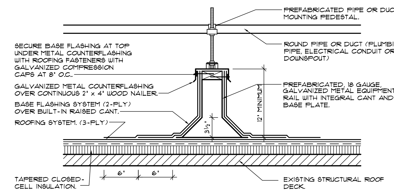
9 PIPE OR DUCT MOUNTING PEDESTAL DETAIL SCALE: 1/2" = 1'-0"
