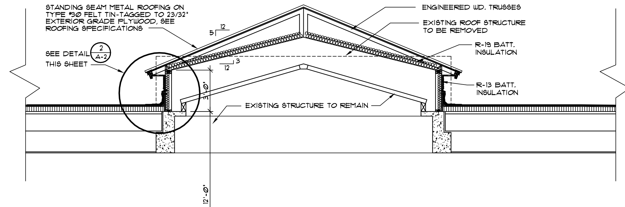
SECTION
