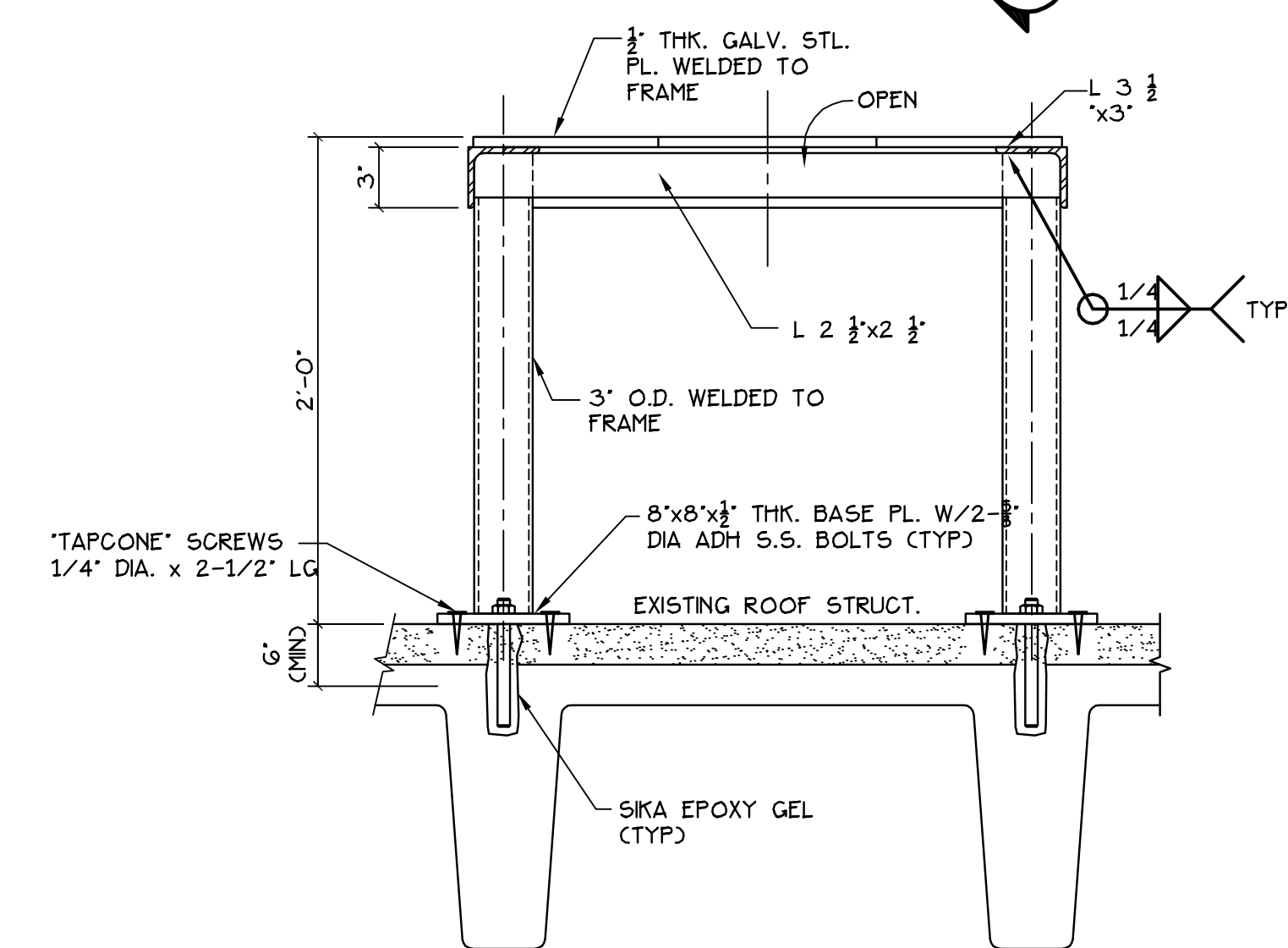
WORKSHOP STEEL EXHAUST PIPE TIE-DOWN DETAIL 2 SCALE: 1 1/2"=1'-0"
