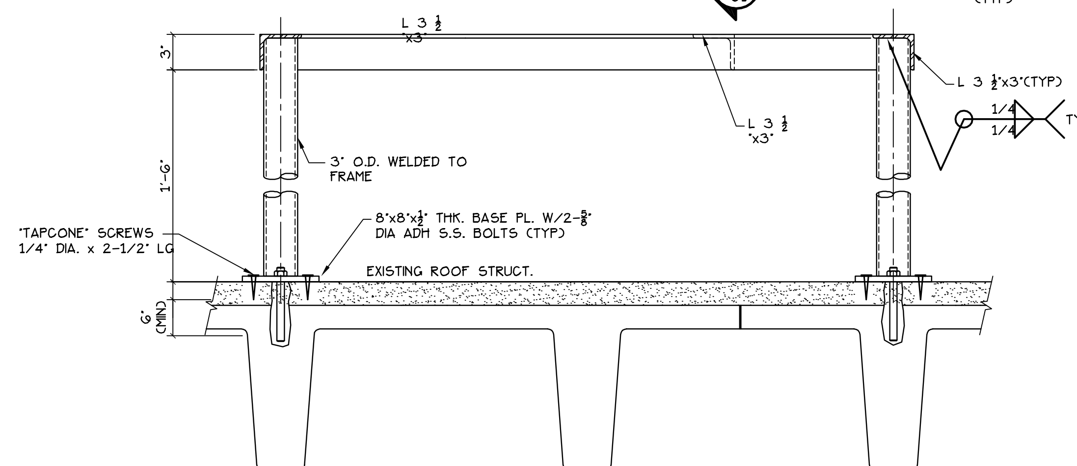
MECHANICAL UNIT SUPPORT DETAIL 4 SCALE: 1 1/2"=1'-0"
