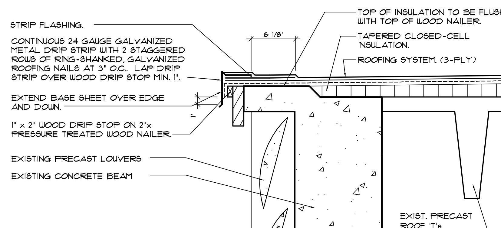
3 A-3 ROOF EDGE DETAIL AT CONCRETE DECK SCALE: 1/2" = 1'-0"
