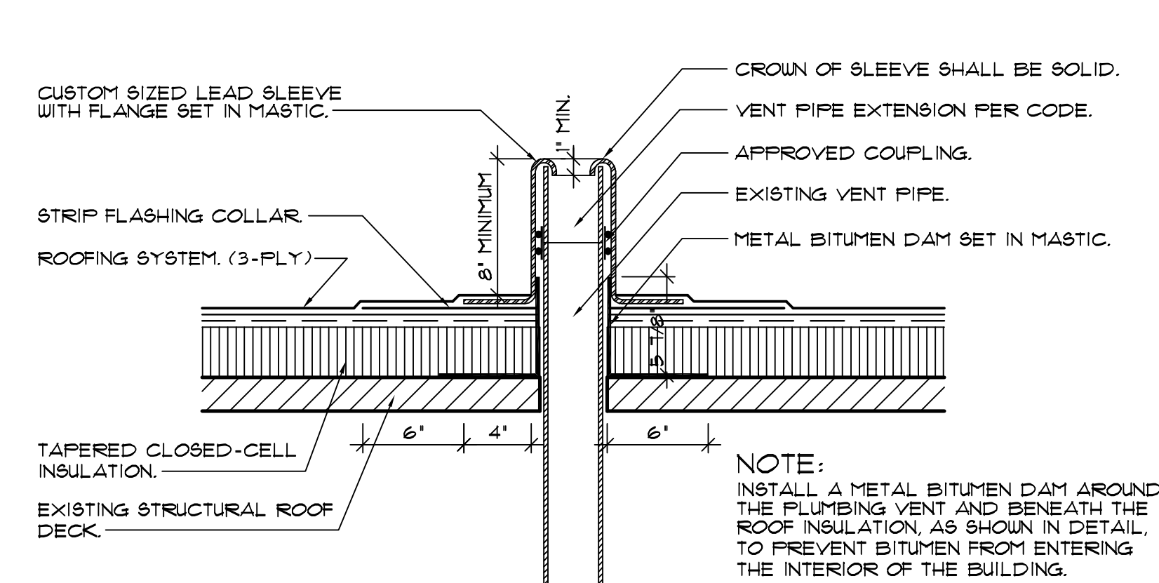
7 PLUMBING VENT DETAIL SCALE: 1/2" = 1'-0"
