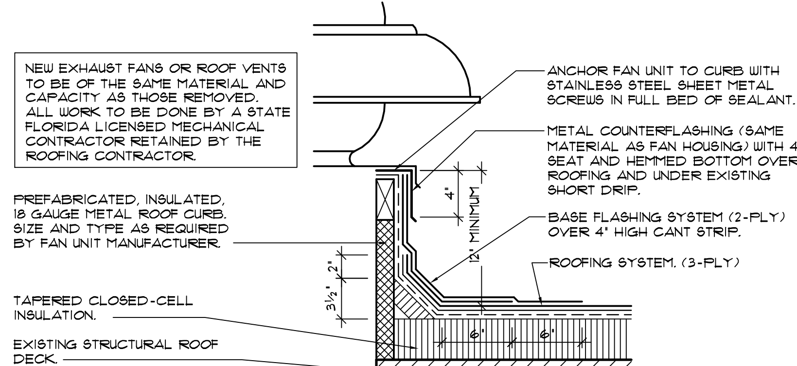
4 A-3 EXHAUST FAN OR ROOF VENT DETAIL SCALE: 1/2" = 1'-0"
