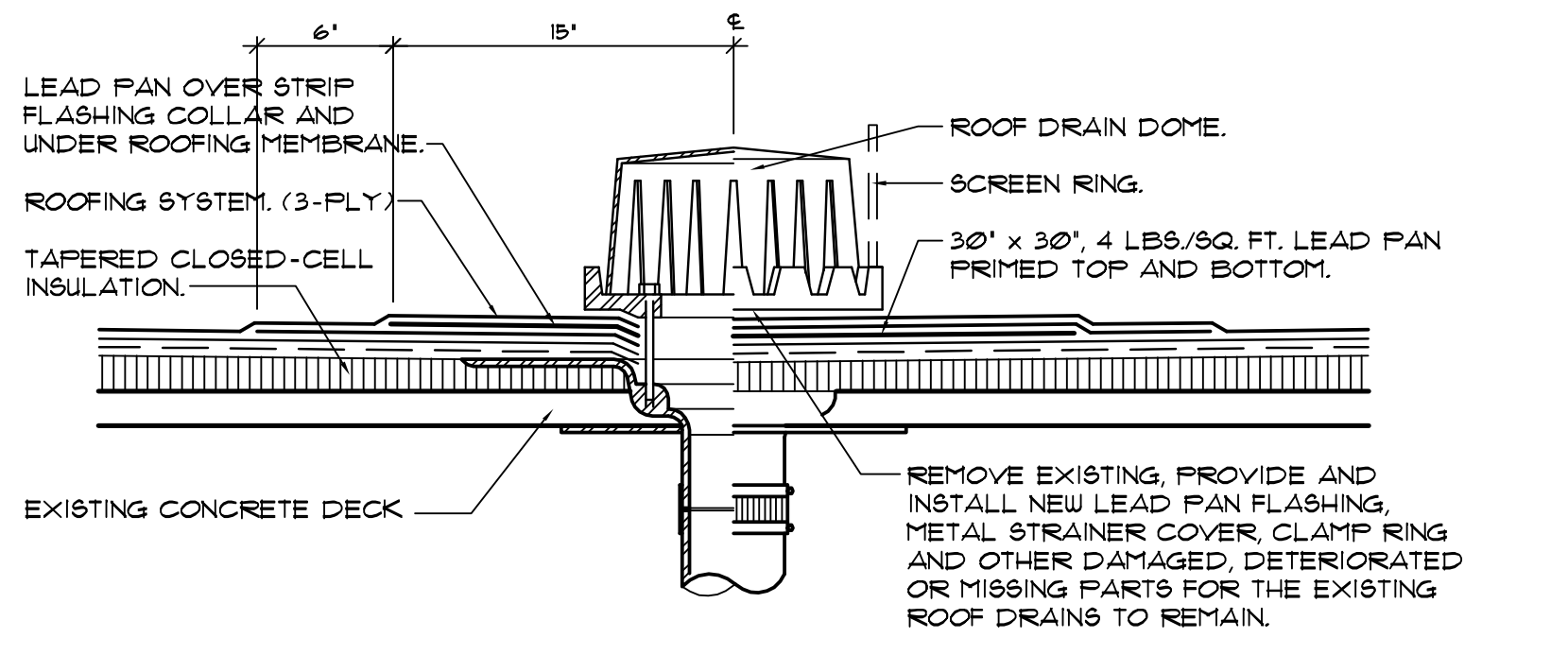
4 ROOF DRAIN DETAIL SCALE: 1/2" = 1'-0"
