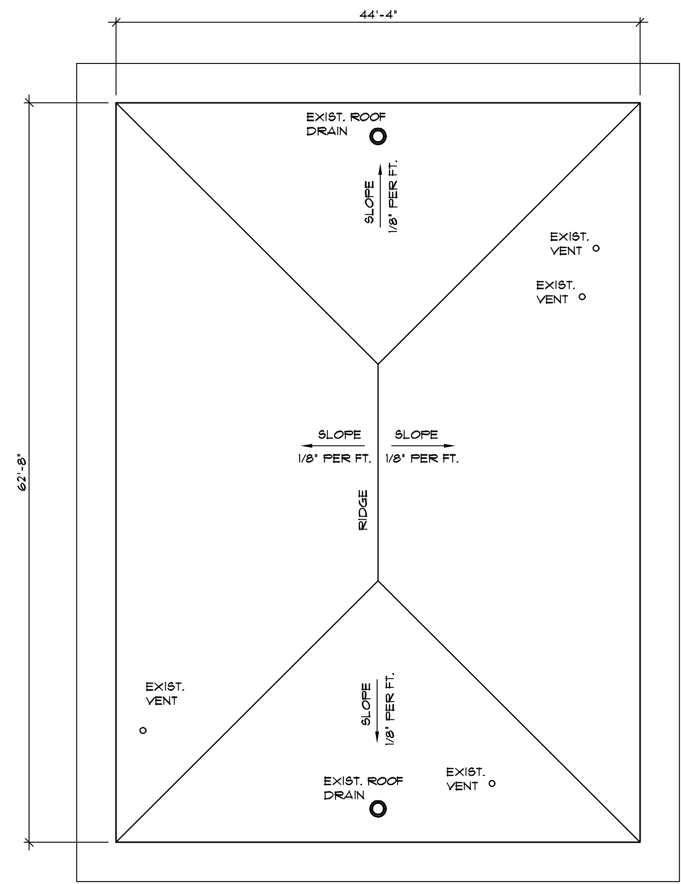
ROOF PLAN BUILDING 'H' SCALE: 1/8" = 1'-0"
