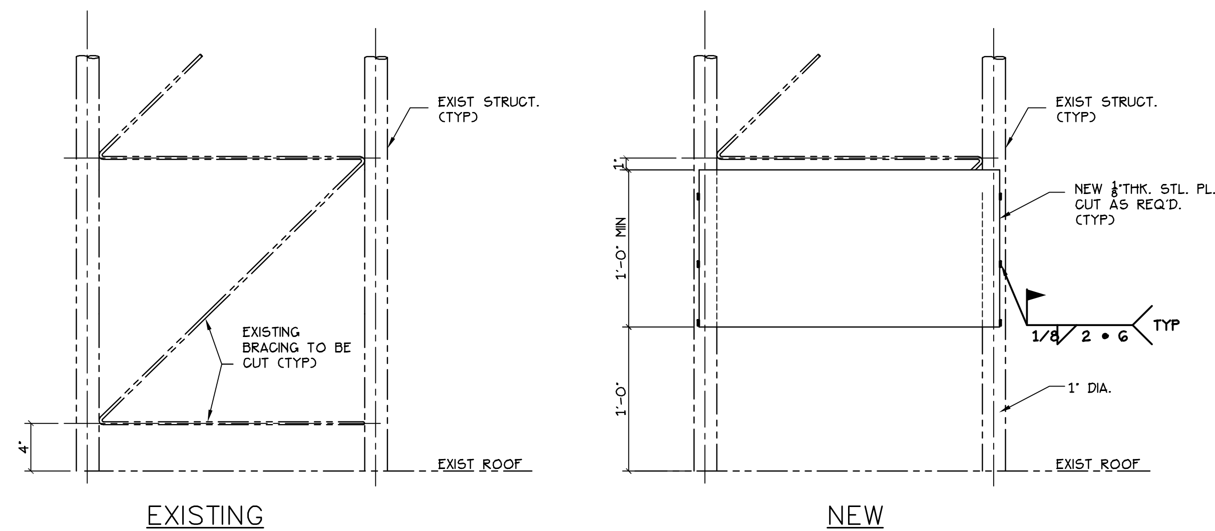
EXIST. RADIO ANTENNA TIE-DOWN DETAIL 1 SCALE: 1 1/2"=1'-0"
