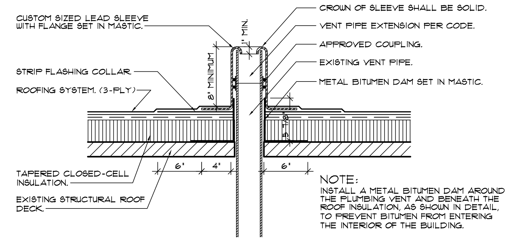
5 PLUMBING VENT DETAIL SCALE: 1/2" = 1'-0"
