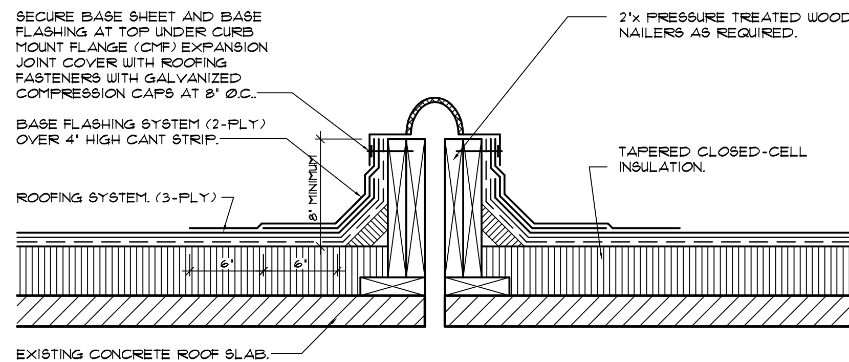
10 EXPANSION JOINT DETAIL SCALE: 1/2" = 1'-0"
