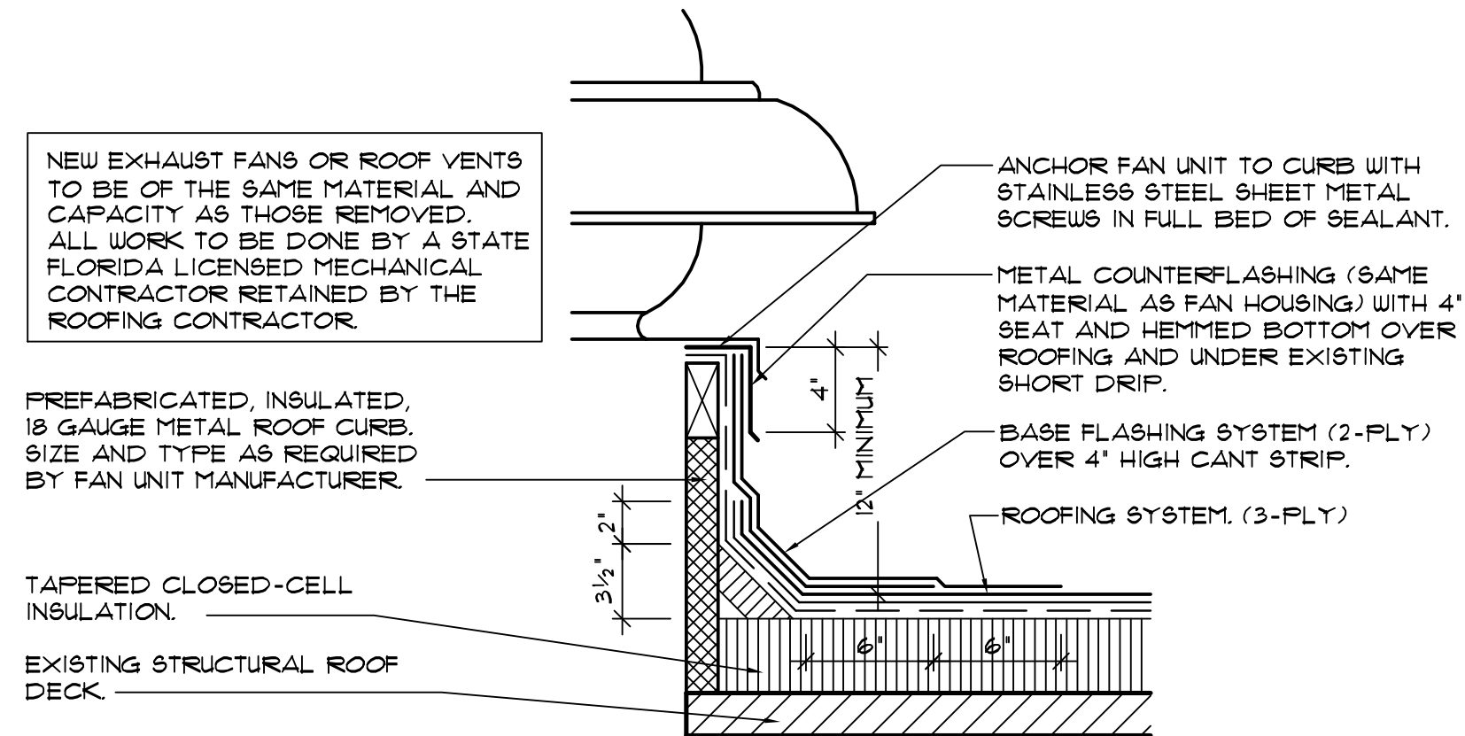
6 EXHAUST FAN OR ROOF VENT DETAIL SCALE: 1/2" = 1'-0"
