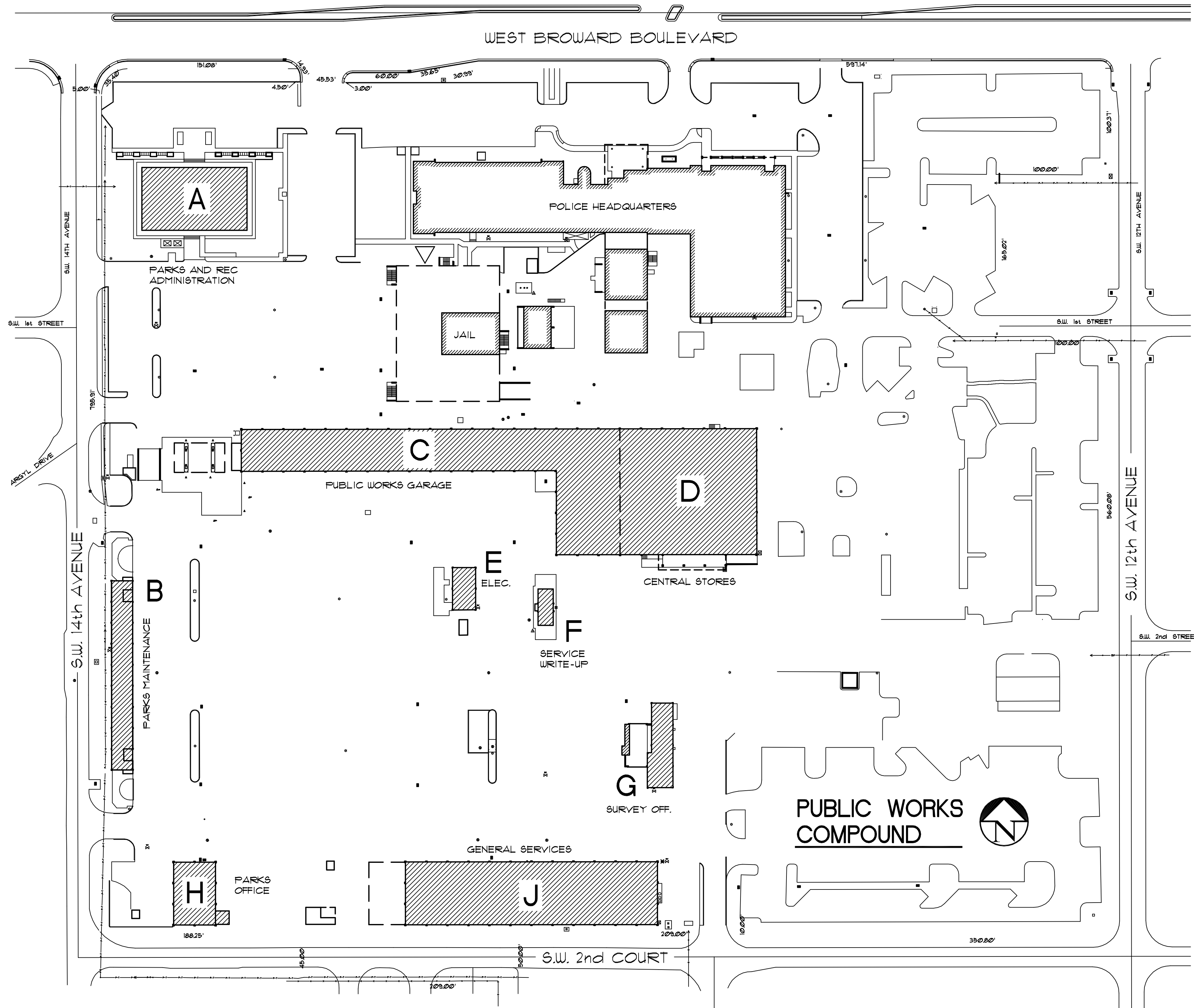
SITE PLAN SCALE 1" = 60'
