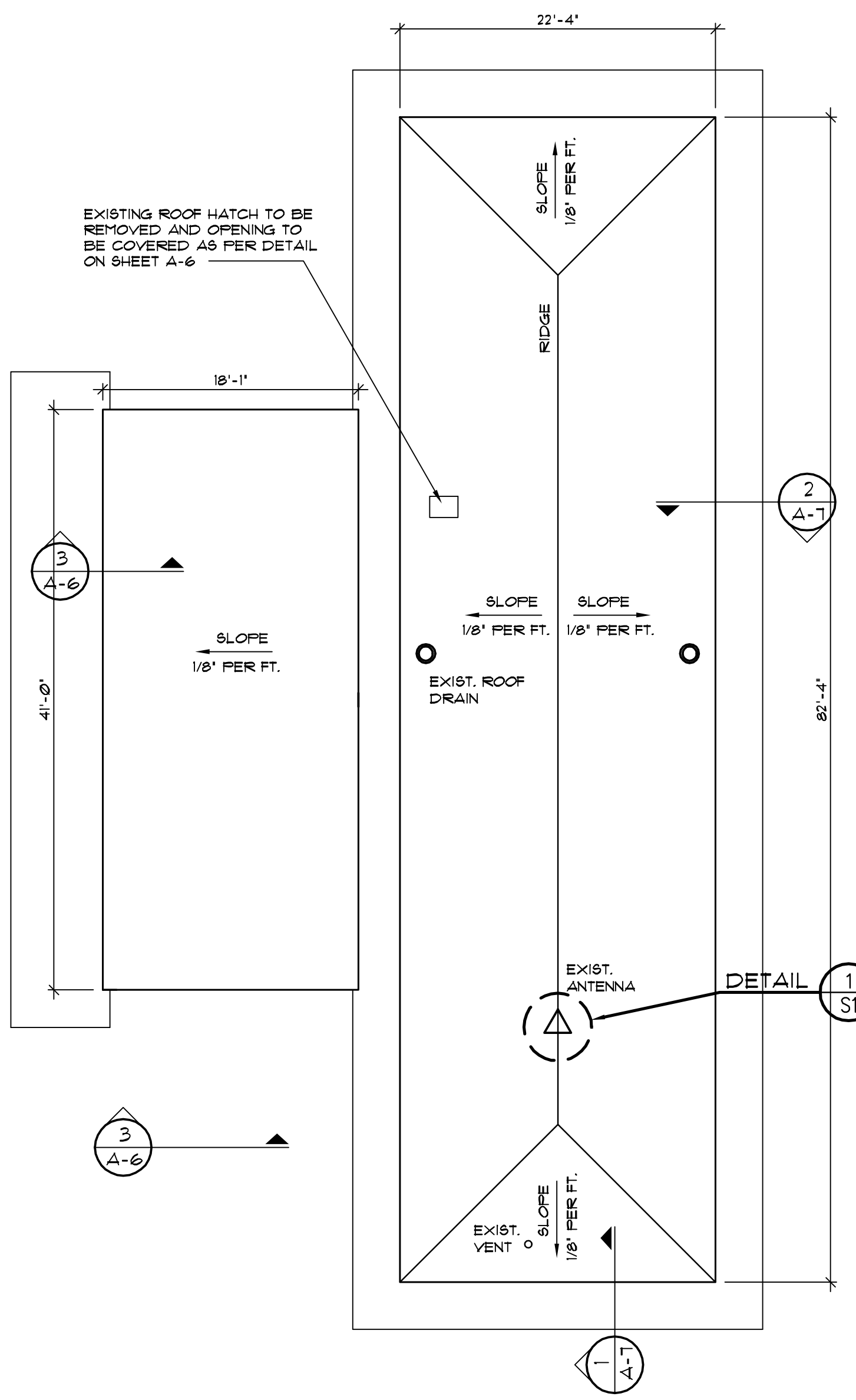
ROOF PLAN BUILDING 'G' SCALE: 1/8" = 1'-0"
