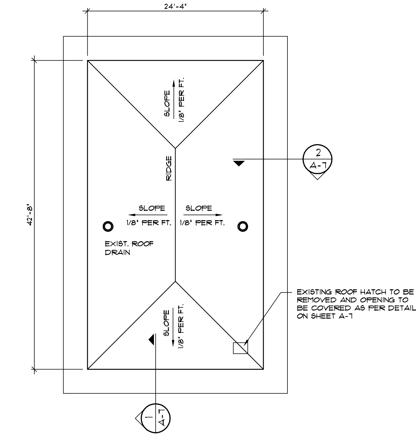
ROOF PLAN BUILDING 'E' SCALE: 1/8" = 1'-0"
