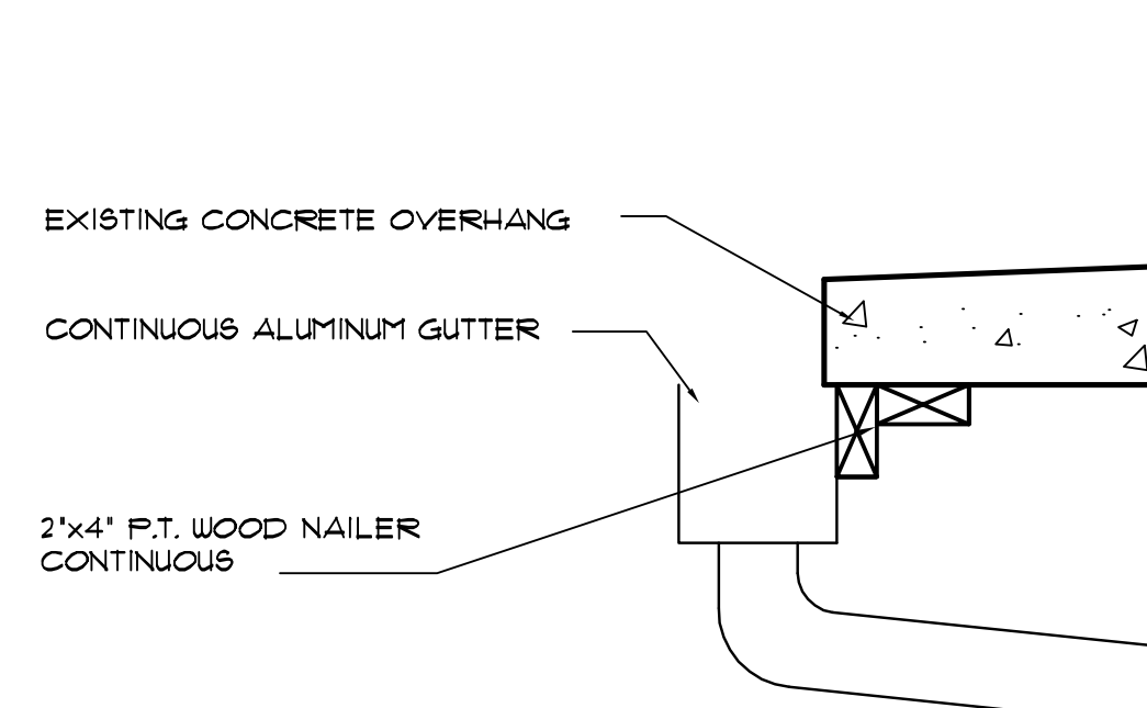
4 GUTTER DETAIL AT CONCRETE OVERHANG SCALE: 1/2" = 1'-0"
