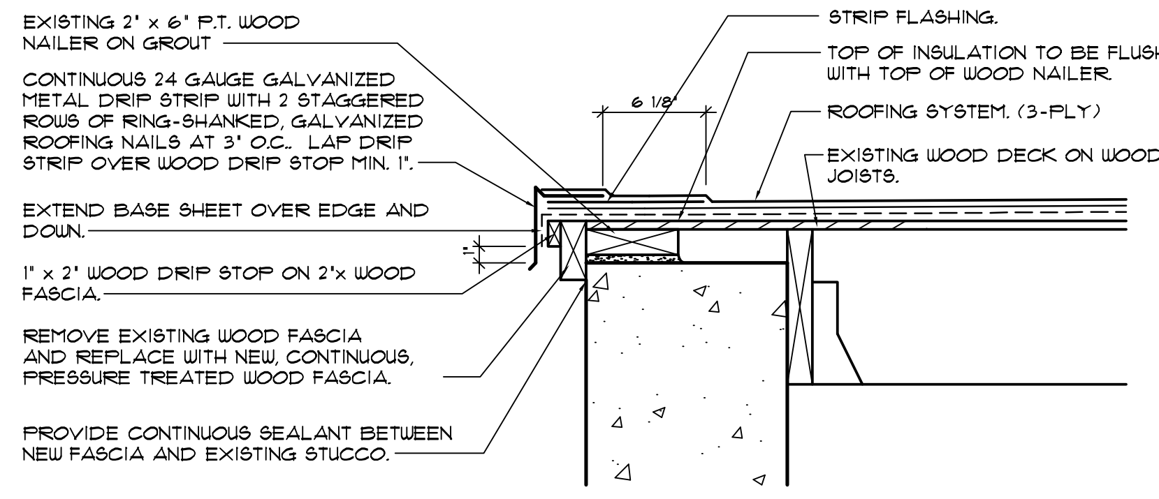
3 ROOF EDGE DETAIL AT WOOD DECK SCALE: 1/2" = 1'-0"
