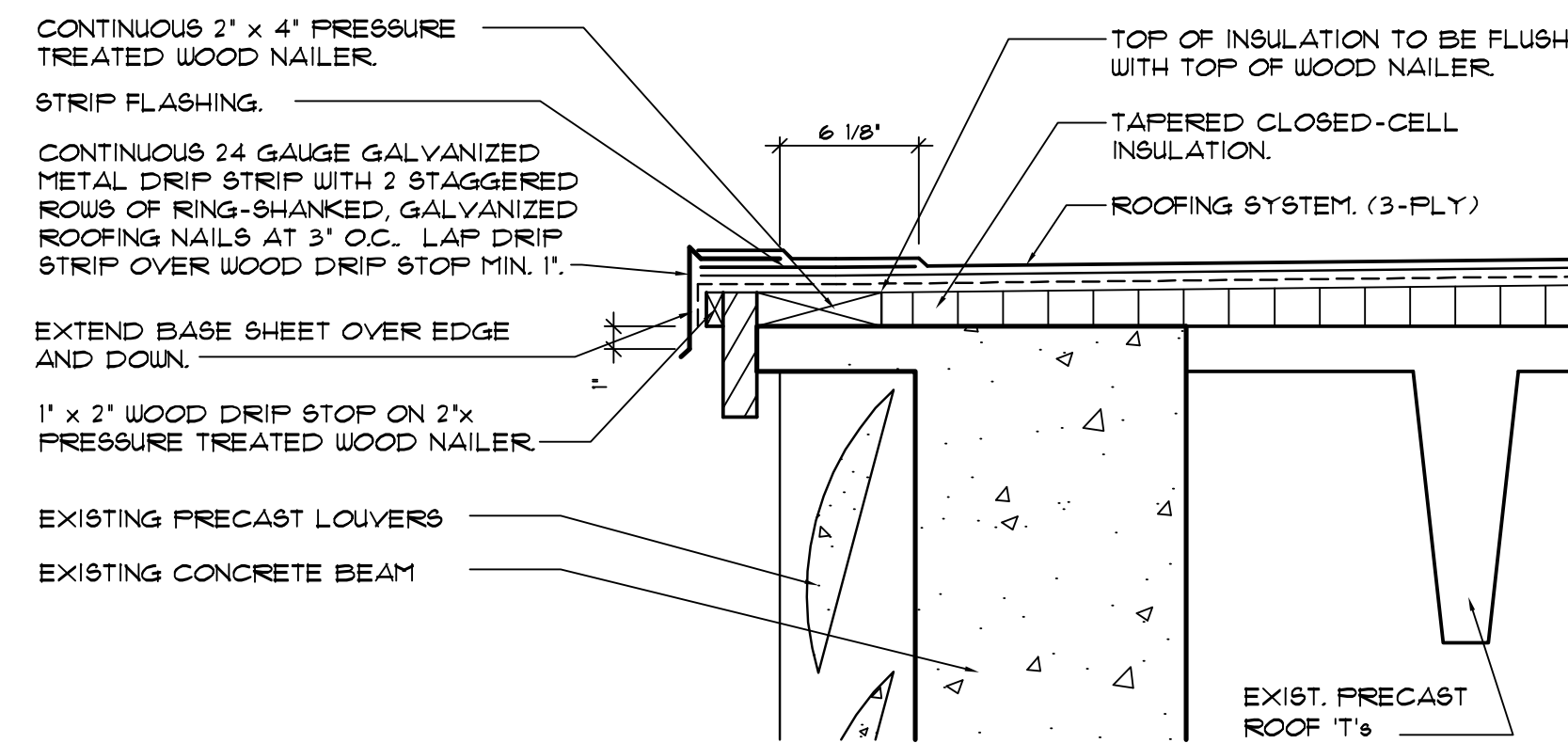
1 ROOF EDGE DETAIL AT CONCRETE DECK SCALE: 1/2" = 1'-0"
