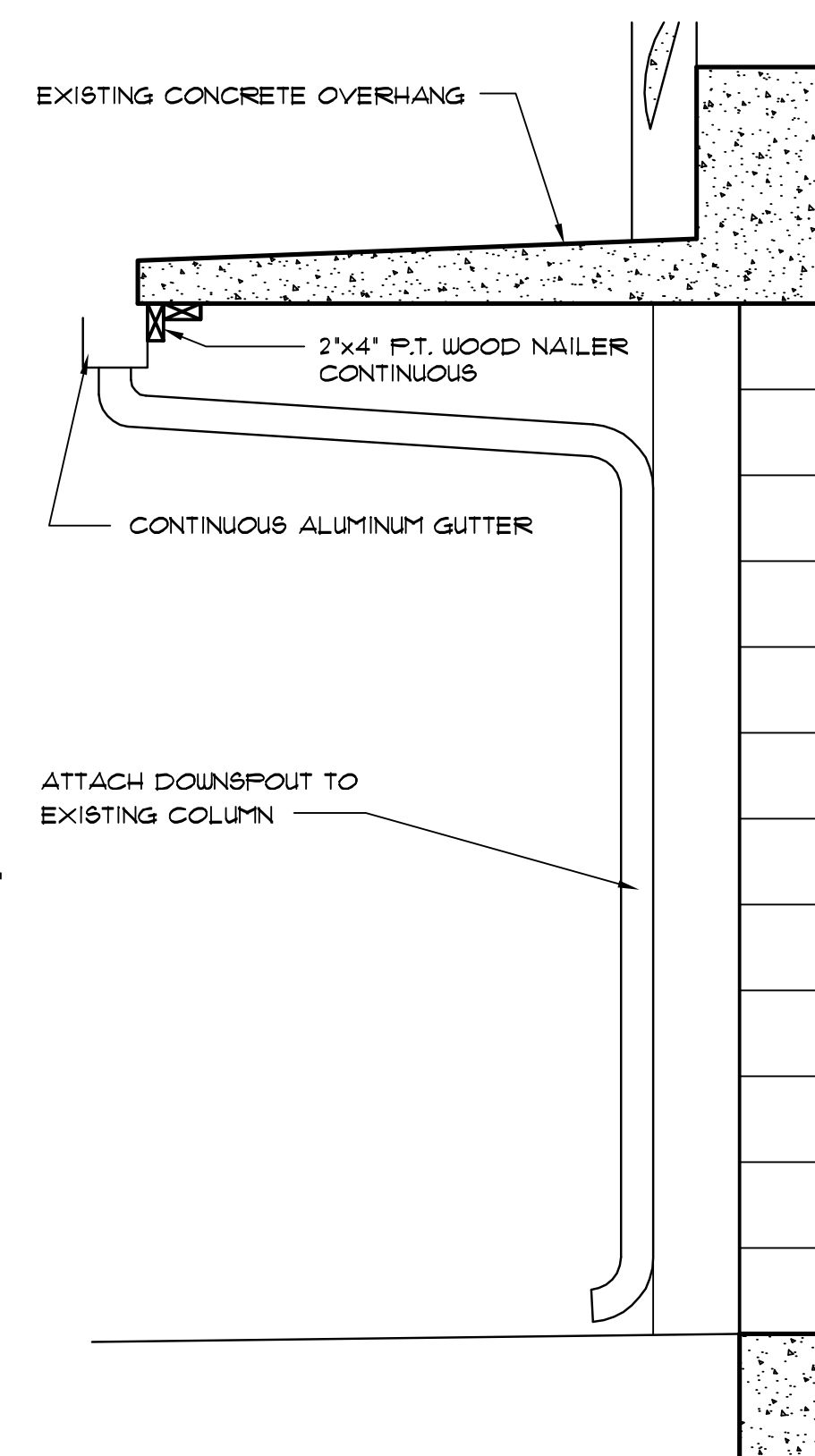
5 A-3 GUTTER DETAIL AT CONCRETE OVERHANG SCALE: 3/4" = 1'-0"
