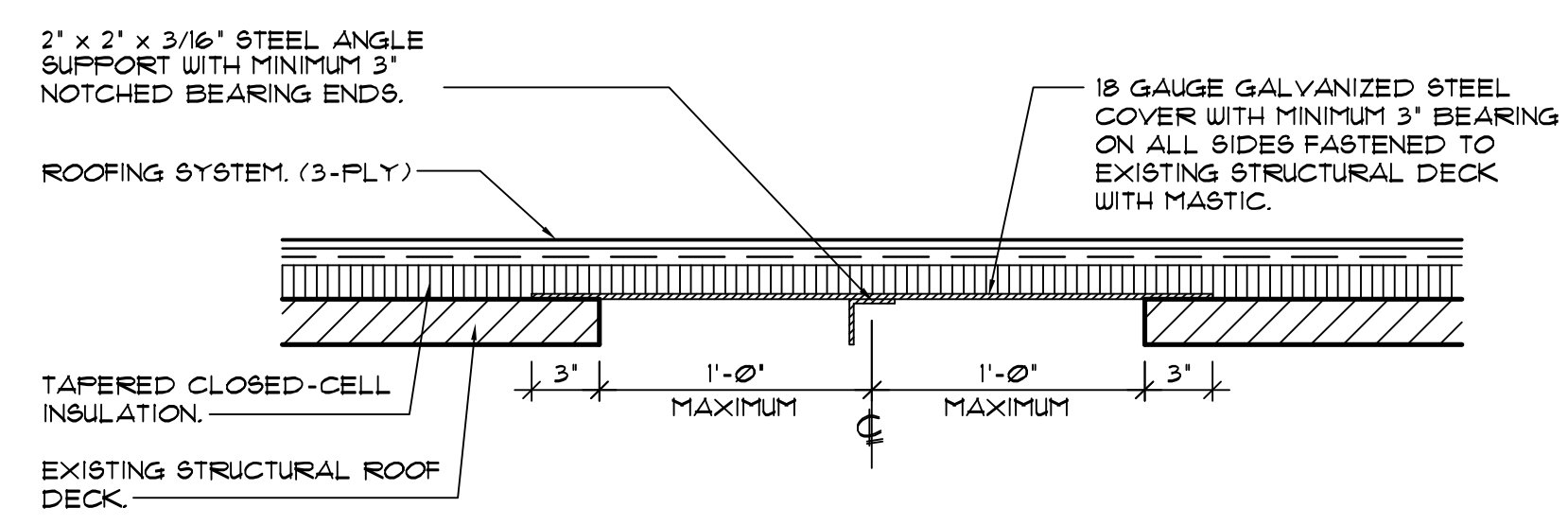
6 TYPICAL DECK OPENING COVER DETAIL SCALE: 1/2" = 1'-0"
