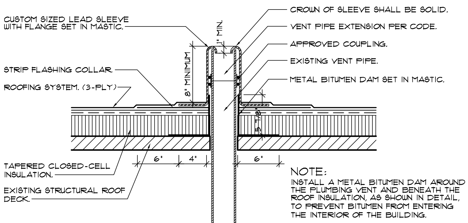
8 PLUMBING VENT DETAIL SCALE: 1/2" = 1'-0"
