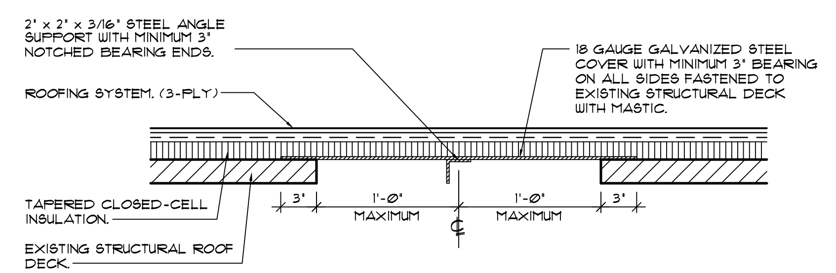
11 TYPICAL DECK OPENING COVER DETAIL SCALE: 1/2" = 1'-0"
