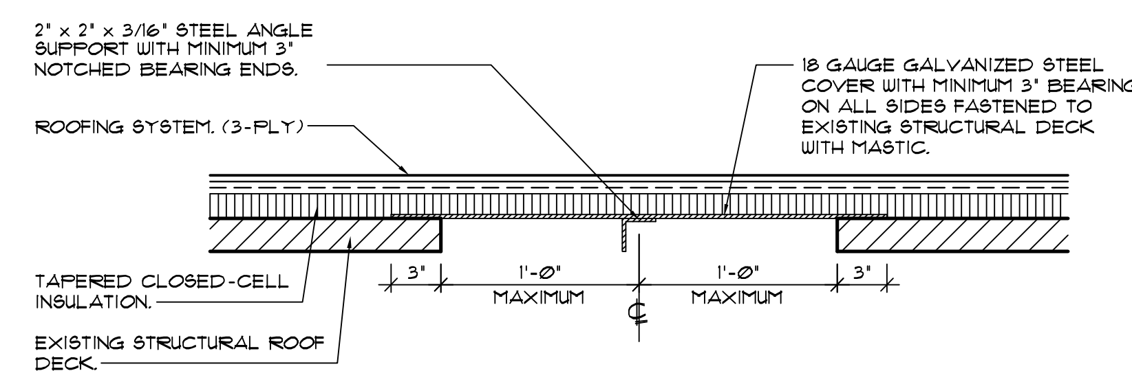
6 A-3 TYPICAL DECK OPENING COVER DETAIL SCALE: 1/2" = 1'-0"
