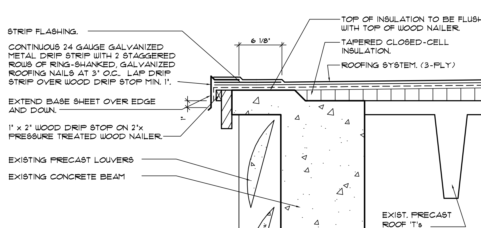
2 ROOF EDGE DETAIL AT CONCRETE DECK SCALE: 1/2" = 1'-0"
