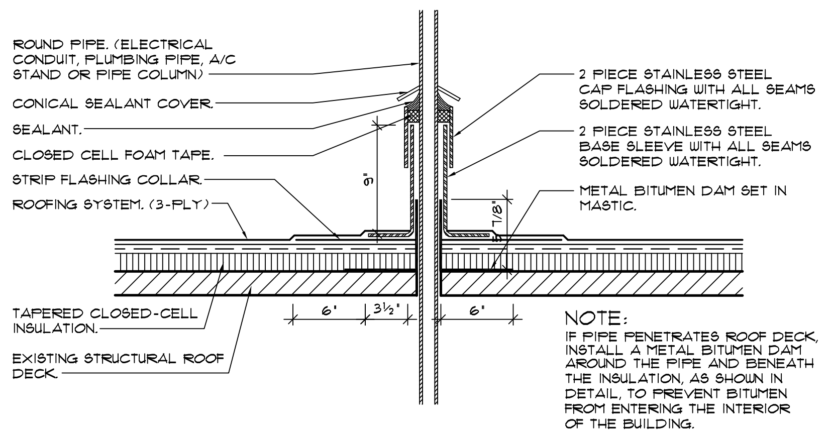
6 CONNECTED PENETRATION DETAIL SCALE: 1/2" = 1'-0"
