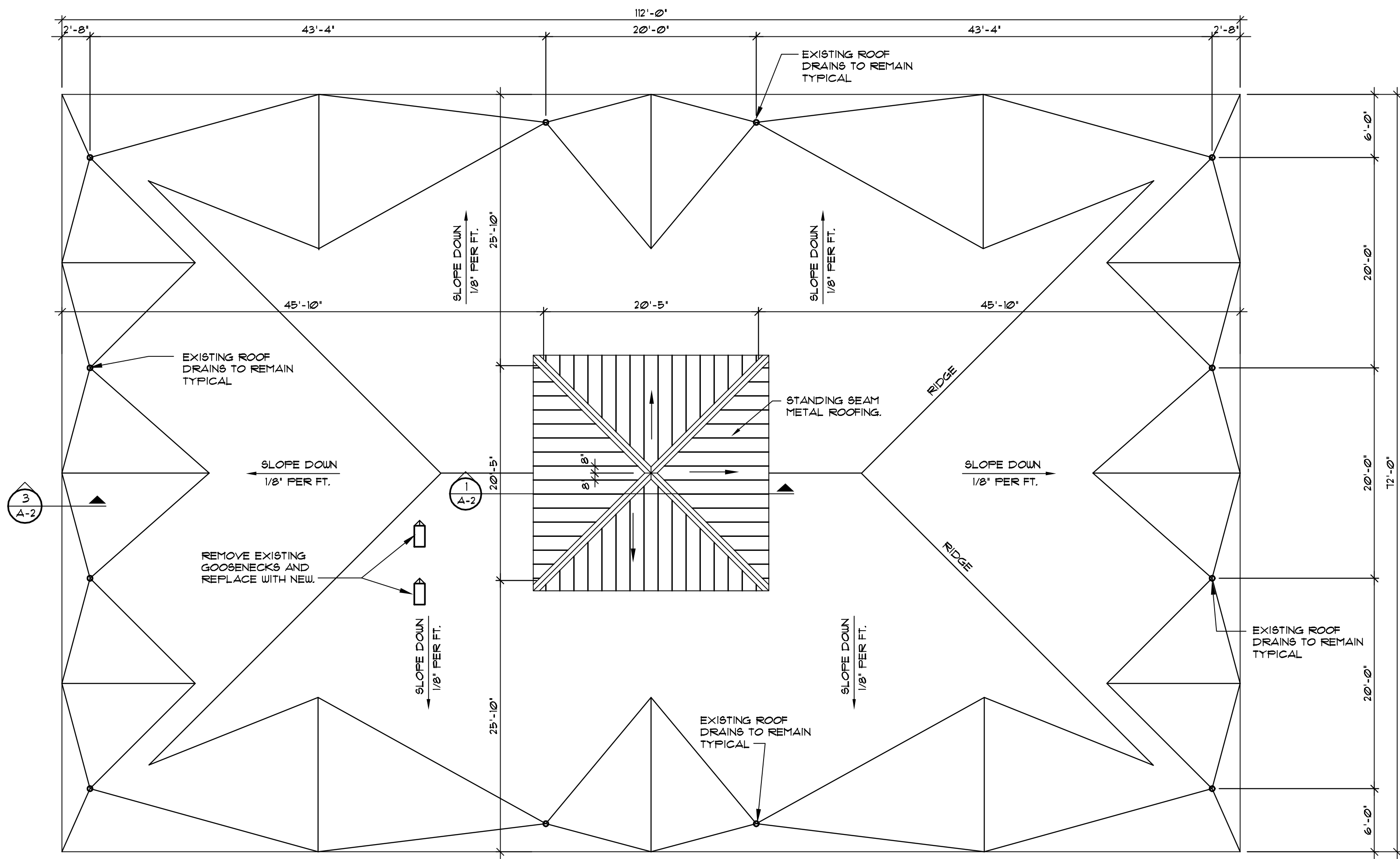
ROOF PLAN
