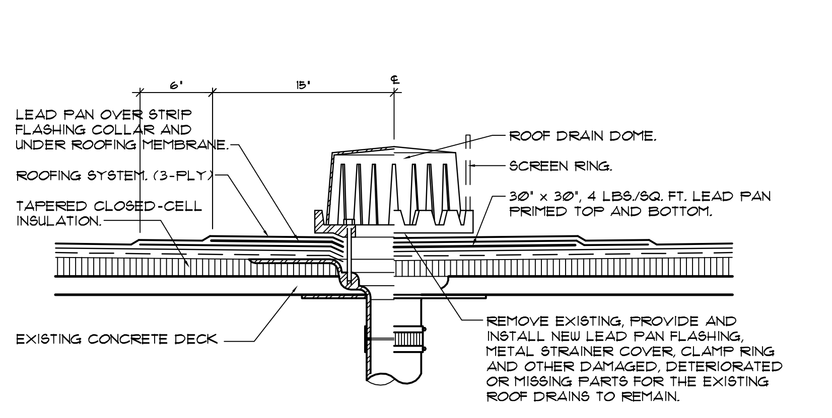
5 ROOF DRAIN DETAIL SCALE: 1/2" = 1'-0"
