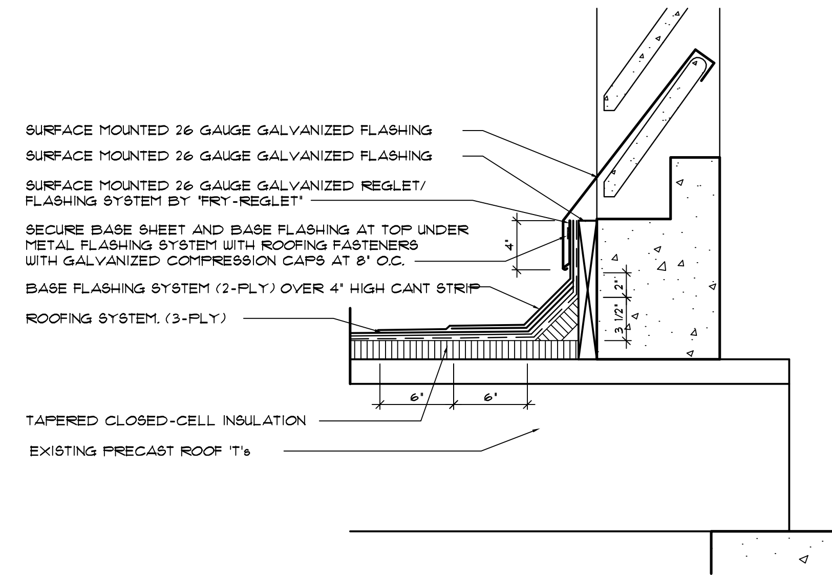
5 STEP DOWN DETAIL AT CONCRETE DECK SCALE: 1/2" = 1'-0"
