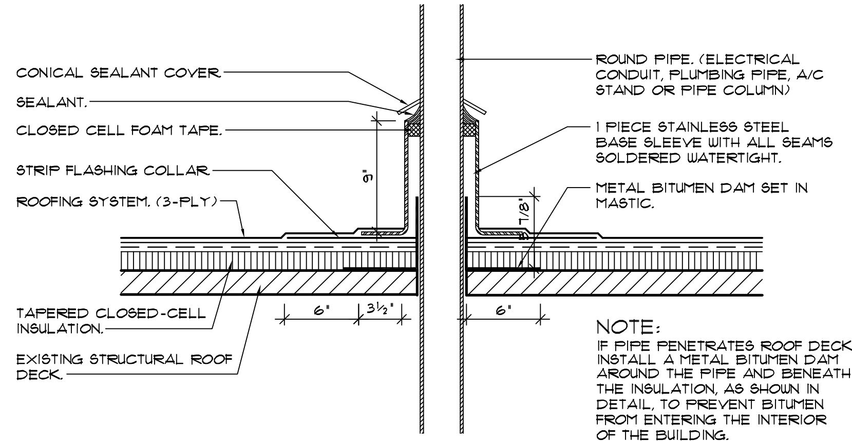
7 DISCONNECTED PENETRATION DETAIL SCALE: 1/2" = 1'-0"
