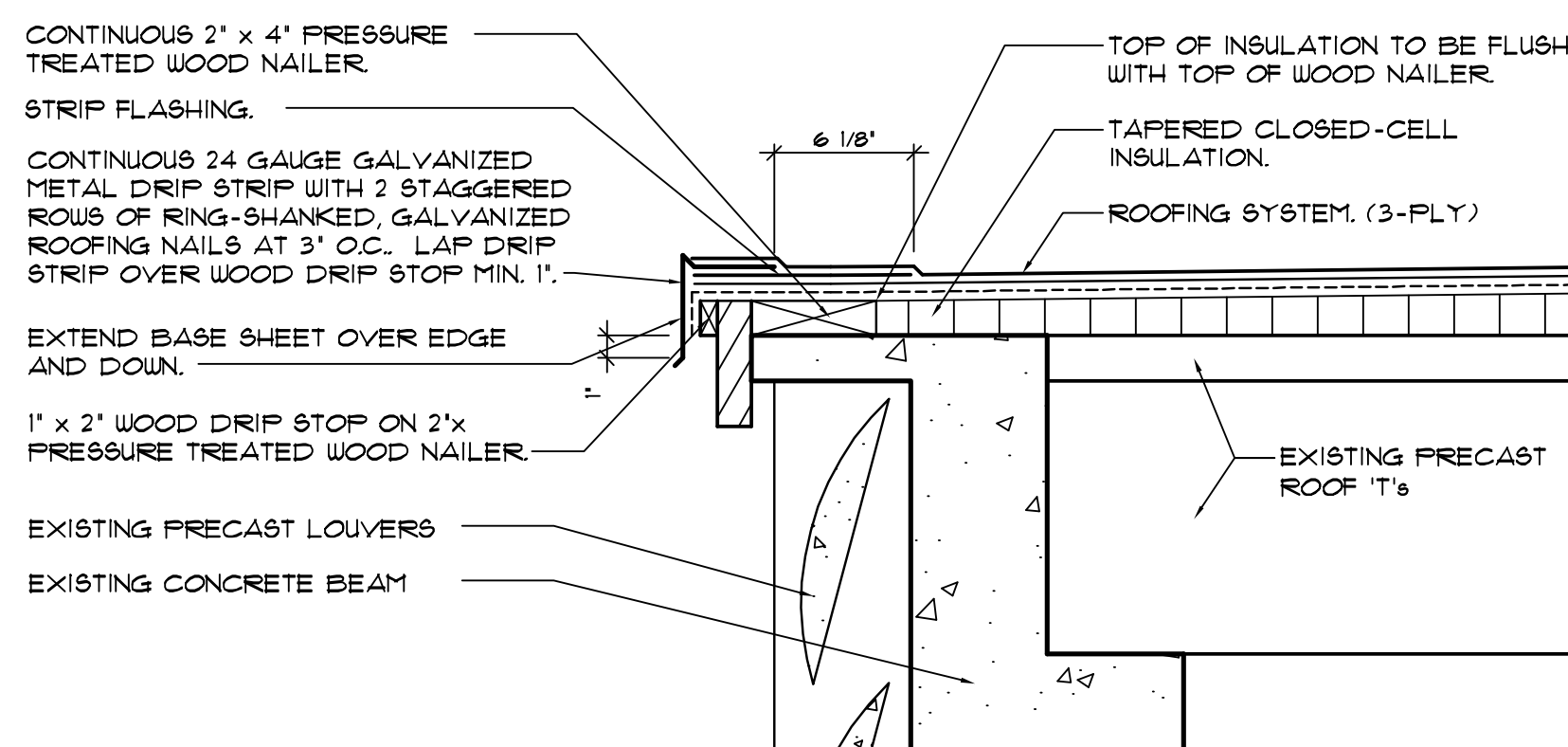
1 A-3 ROOF EDGE DETAIL AT CONCRETE DECK SCALE: 1/2" = 1'-0"
